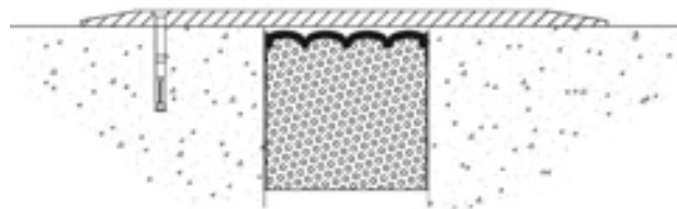
Horizontal Colorseal is typically installed in an area where vehicular or pedestrian traffic does not come in direct contact with the seal. In required vehicular situations it can be installed in conjunction with a metal coverplate, however Sika Emseal recommends the SJS system (see page 22).
