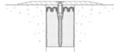
SJS is now available for joint sizes as small as 2" (50mm).
