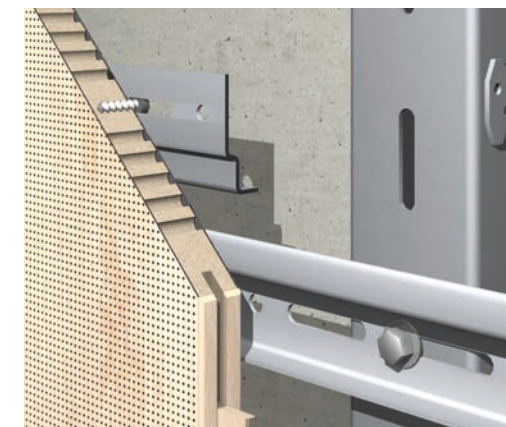
detailed view: vertical mounting with spring
