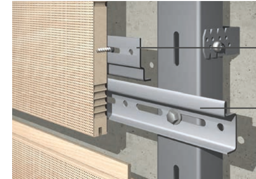
detailed view: horizontal mounting with spring
