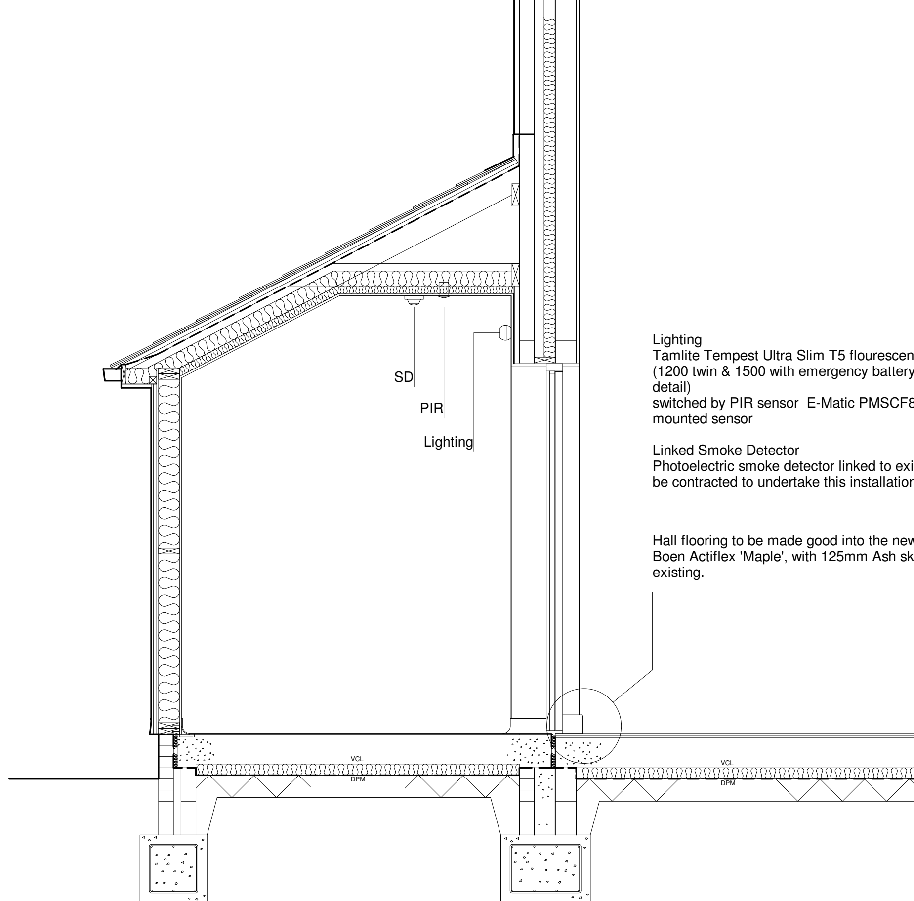
Detail Section Through New door opening
