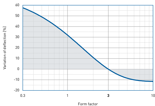
Deflection
