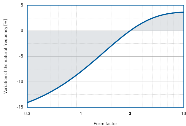
Natural frequency
