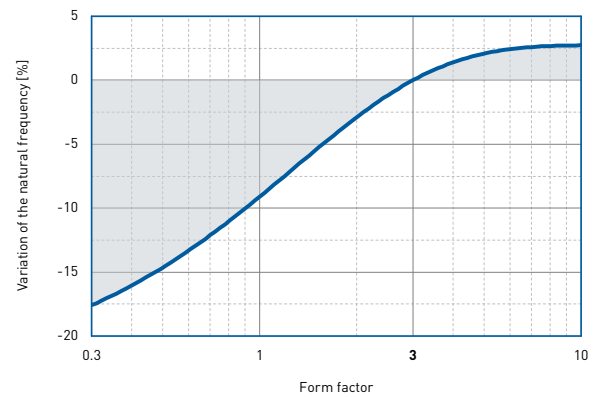
Natural frequency
