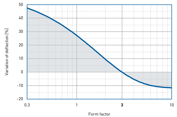
Deflection
