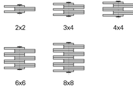
Plate lacing
