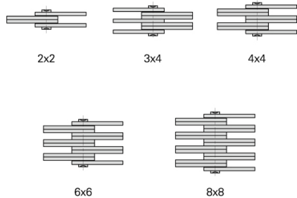
Plate lacing
