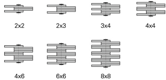
Plate lacing
