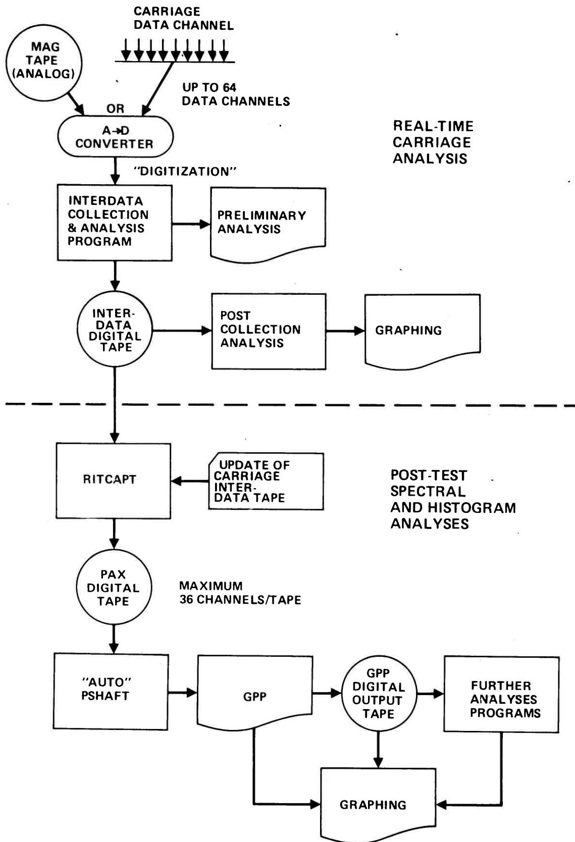
Figure 5 - Flow Chart for Computer Analysis
