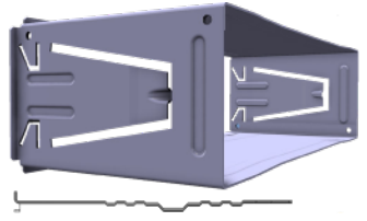
1-DIN Sized Mounting Frame & Removal Tools. Suits for all 1-DIN devices.
