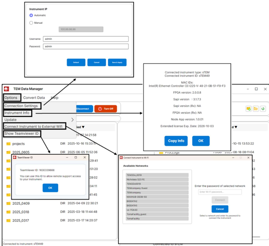
Figure 37: General Options menu
