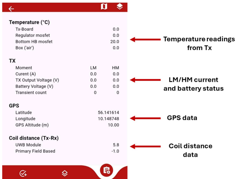
Figure 34: Additional information tab
