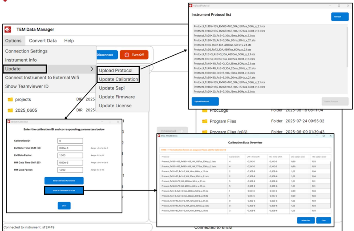
Figure 38: Update menu in TEM Data Manager
