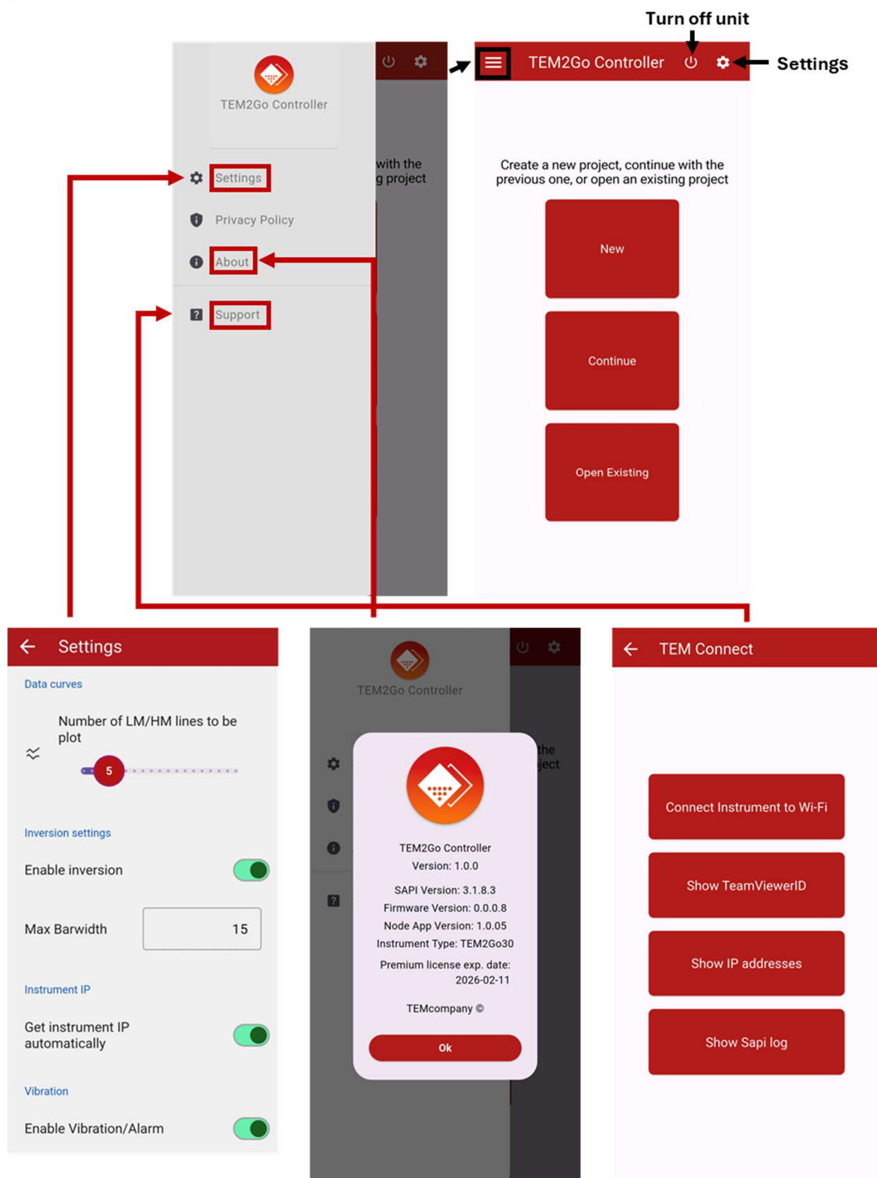
Figure 30: TEM2Go Controller App environment start-up and menu.
