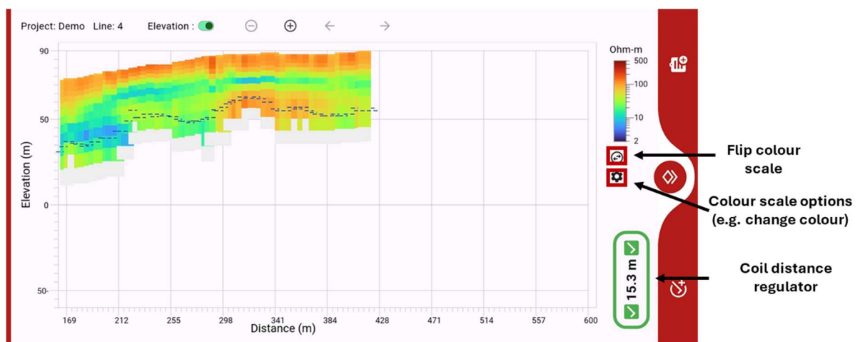
Figure 35: Real-time inversion tab. You can see a pseudo-2D resistivity section of several 1D interpolated models measured in a line. DOI is shown as the dotted lines.
