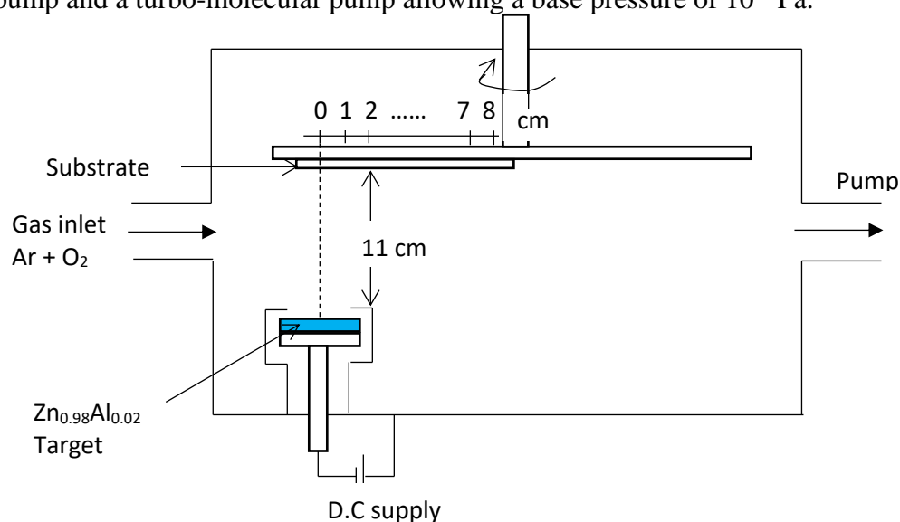
Figure 1: Schematic representation of the sputtering chamber.
