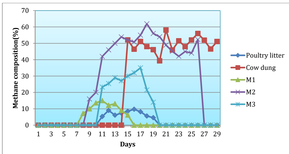
Figure 3: Methane percentage composition per substrate
