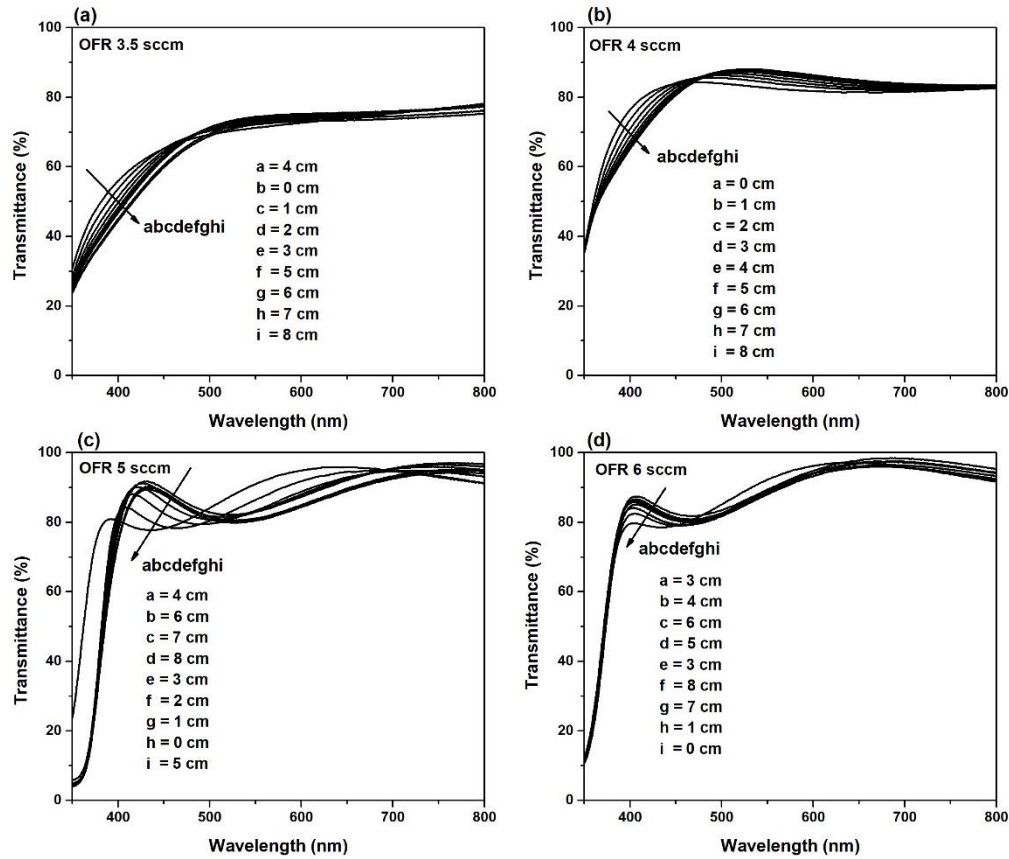
Figure 3: Variation of transmittance of AZO films with substrate positions for different oxygen flow rates (a) OFR 3.5 (b) OFR 4 (c) OFR 5 and (d) OFR 6 sccm.
