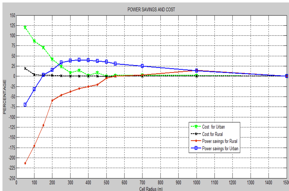
Figure 2: Percentage power savings and cost vs Cell radius
