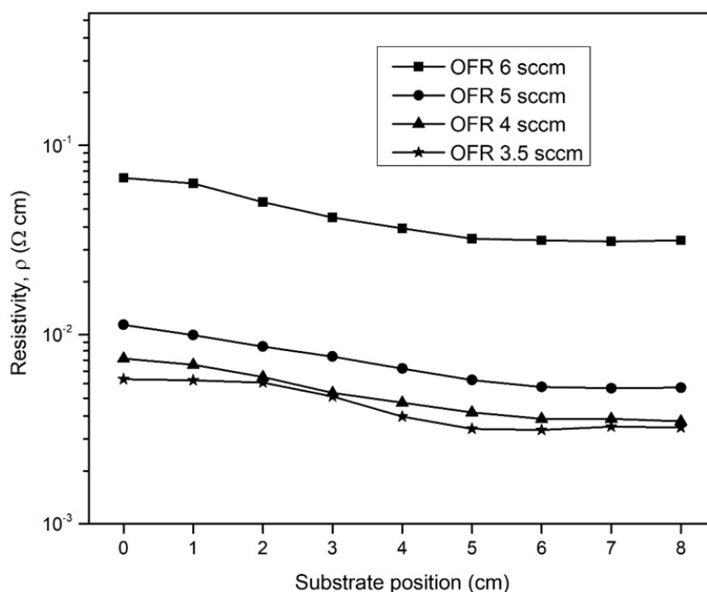
Figure 2: Resistivity of AZO films for different oxygen gas flow rates (OFR).
