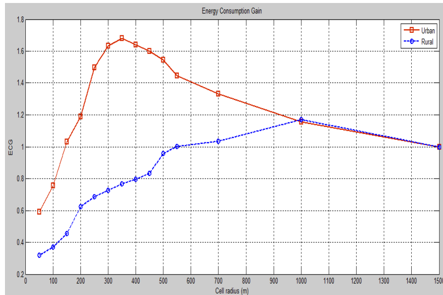
Figure 3: Energy Consumption Gain vs Cell radius
