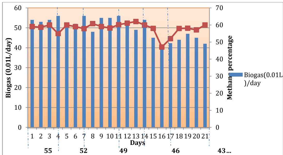
Figure 3: Biogas output and methane % variation with temperature for reactor B
