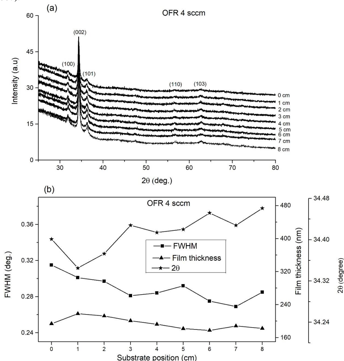
Figure 5: (a) X-ray diffraction spectra (b) FWHM, 2\theta (of the (002) peak) and film thickness of AZO films as a function of substrate position for the optimum OFR of 4 sccm.
