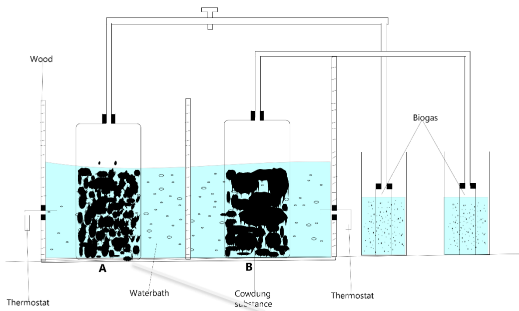
Figure 1: Experiment set up
