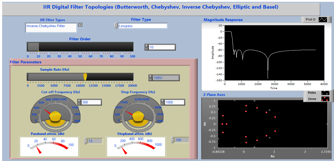
Figure 10: UI showing Magnitude response and Pole-Zero Plot of a 10th Order Inverse Chebyshev Filter
