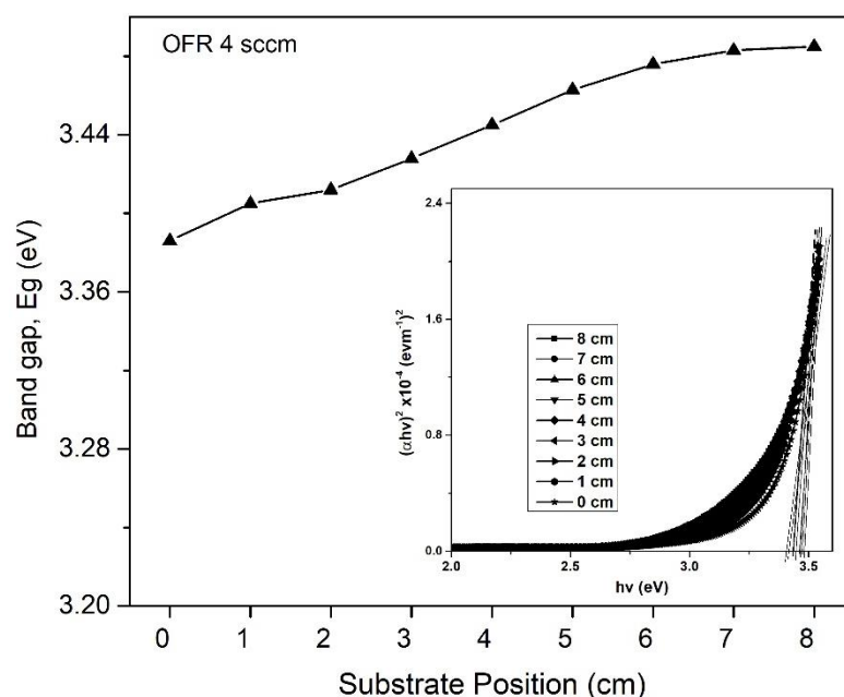
Figure 4: Evolution of band gap with substrate position for optimized AZO films obtained with the optimum OFR of 4 sccm. Inset is Tauc's plot of (ahv)^2 versus h\nu used to determine the band gap.
