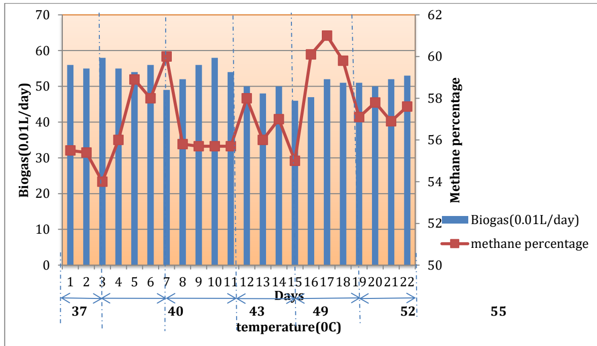
Figure 2: Biogas output and methane % variation with temperature for reactor A
