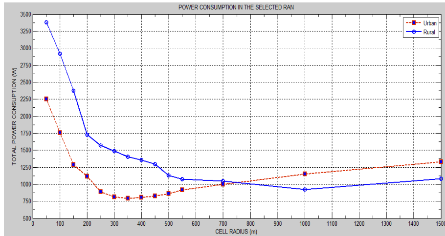
Figure 1: Total power consumption vs Cell radius
