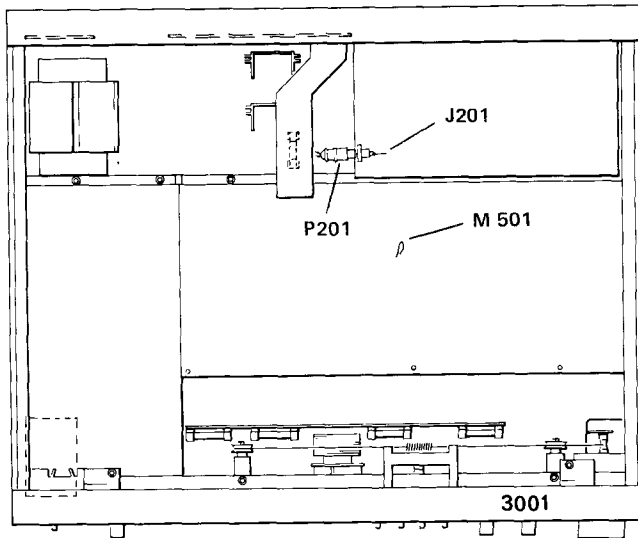
Figure 25 Test points
