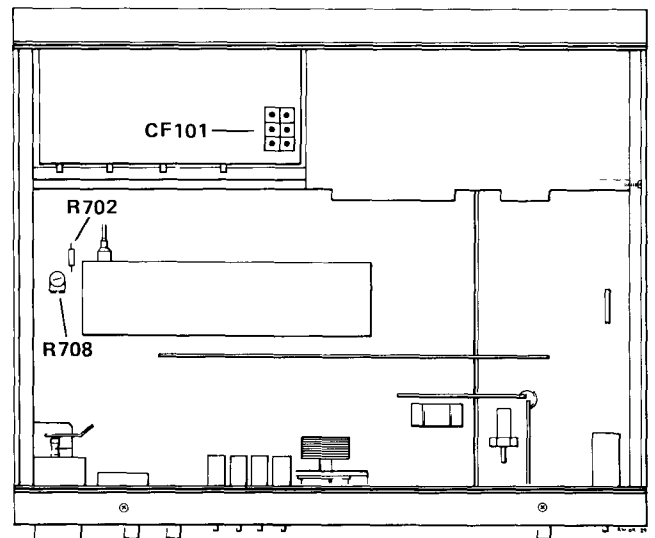
Figure 32 Test points
