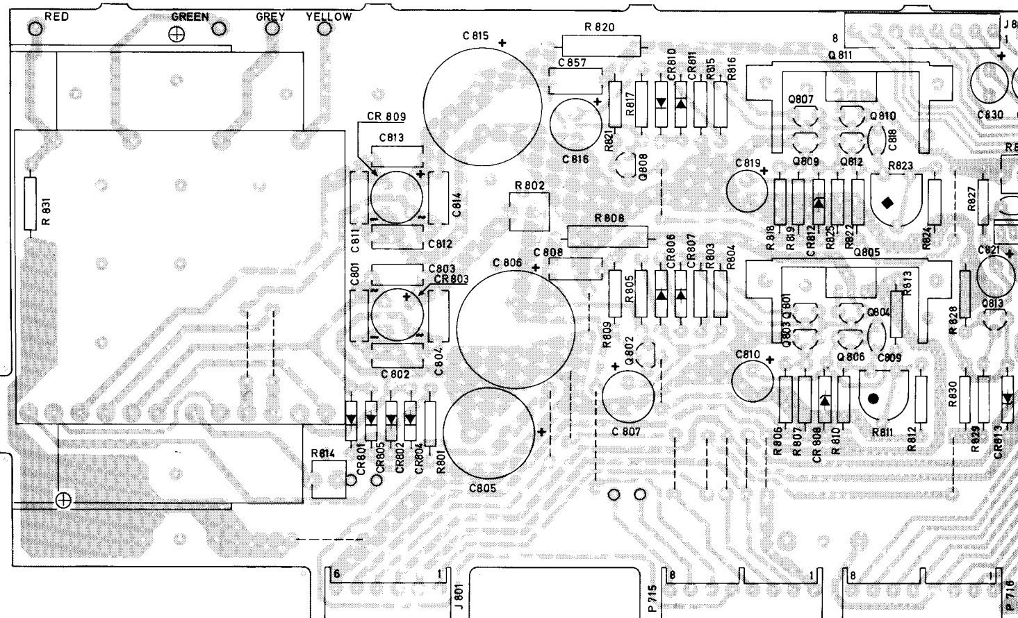
Figure 10 Power supply board, component side
