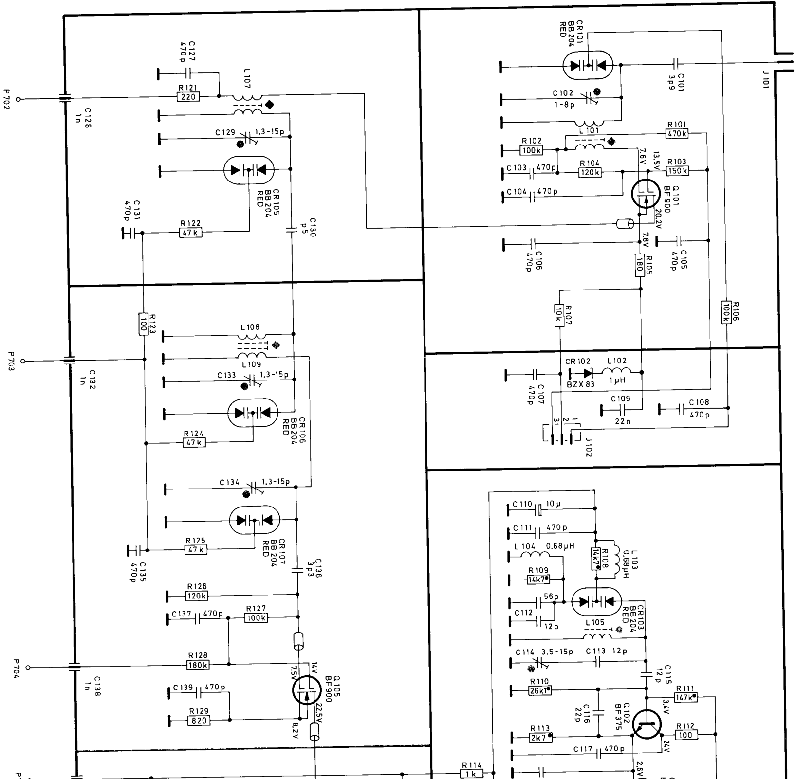
Figure 12 Front end
