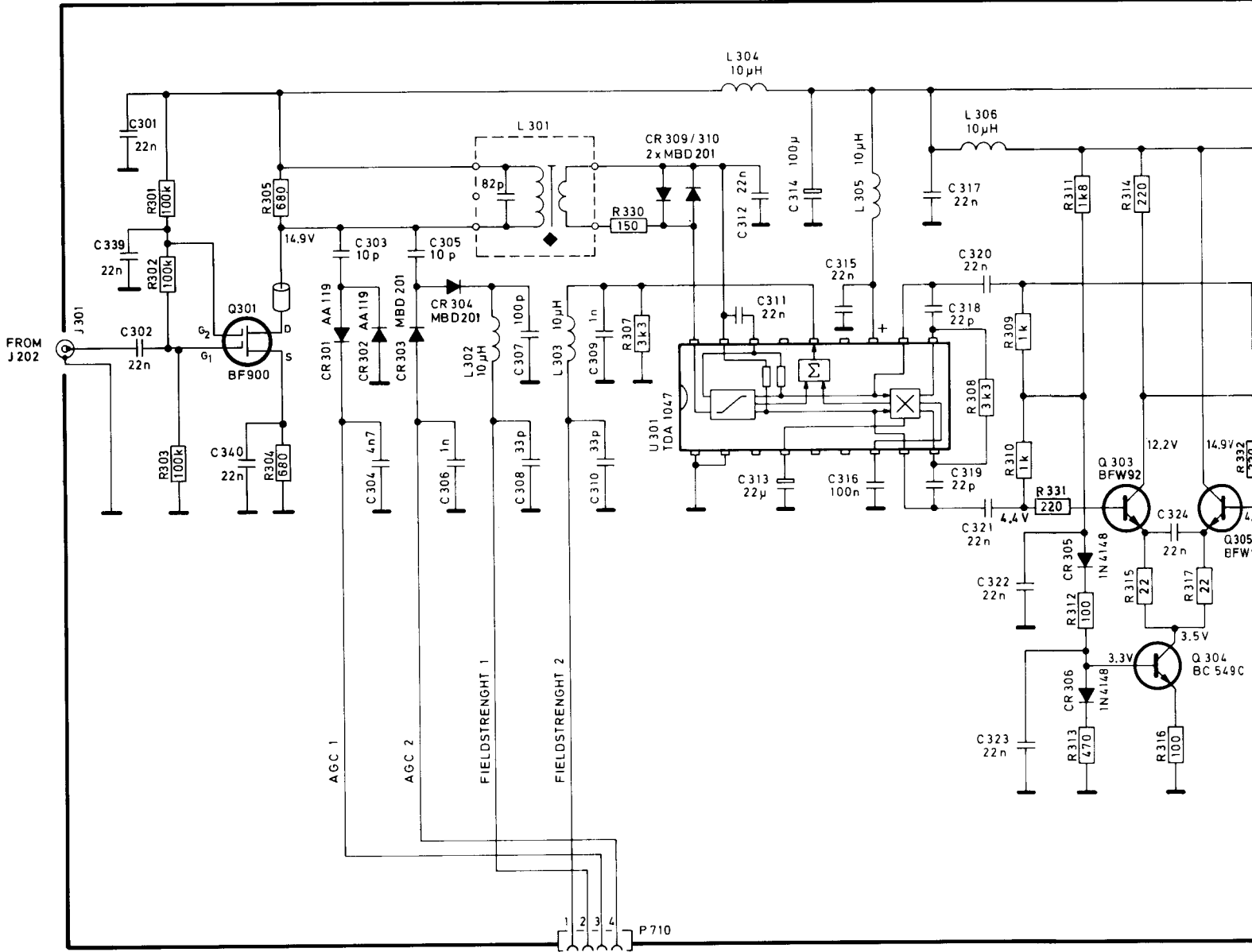
Figure 22 Limiter/detector above serial No. 00700
