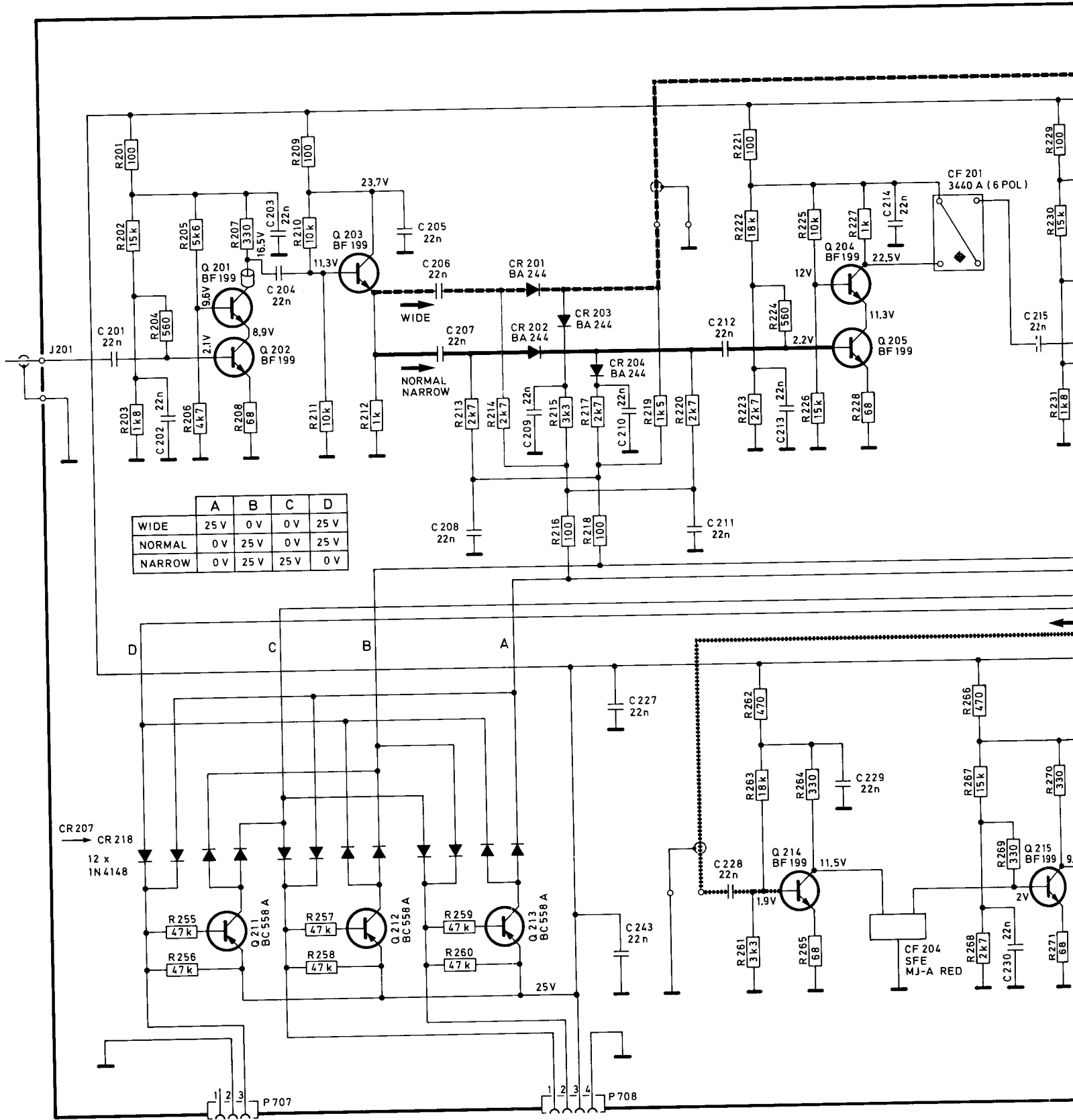
Figure 28 Selectivity circuit, below serial No. 00700
