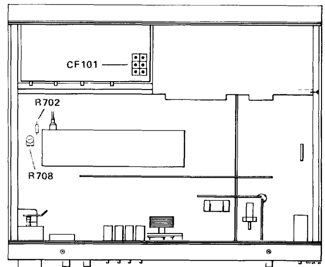
Figure 37 Test points
