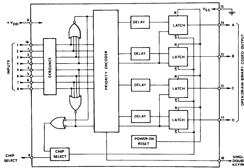
U1004 MC14430
