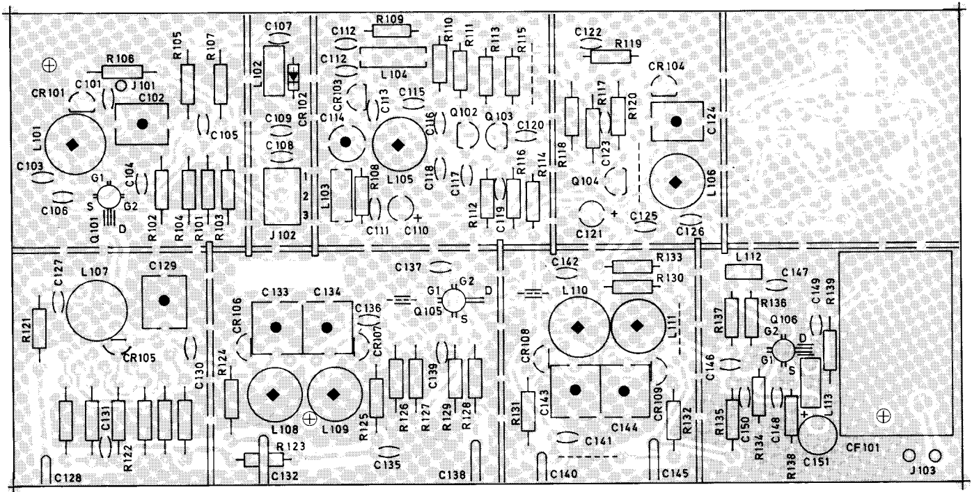
Figure 14 Front end board, component side
