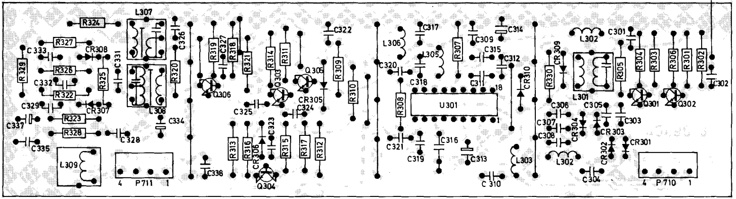
Figure 17 Limiter/detector board below serial No. 00700, foil side
