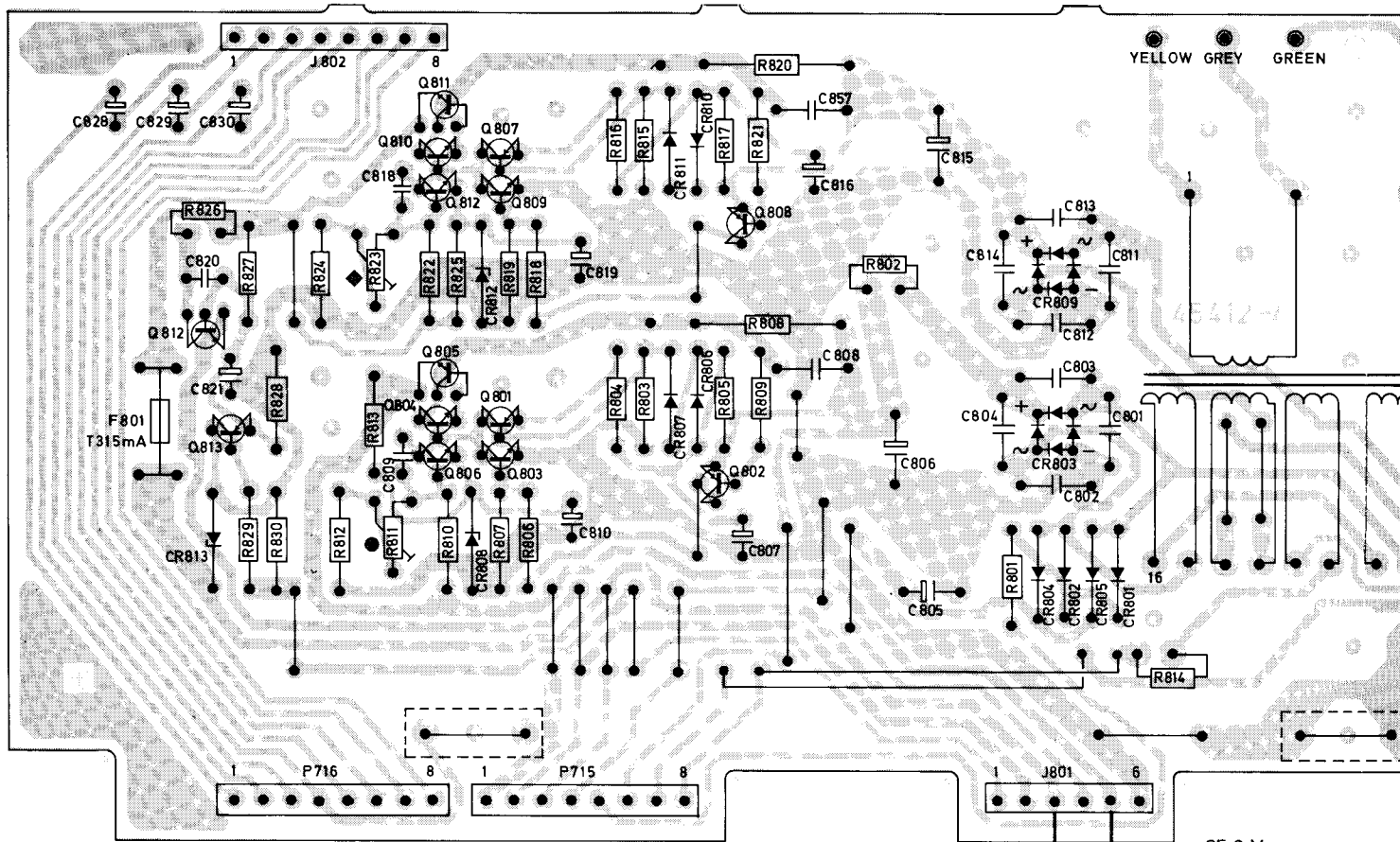
Figure 9 Power supply board, foil side
