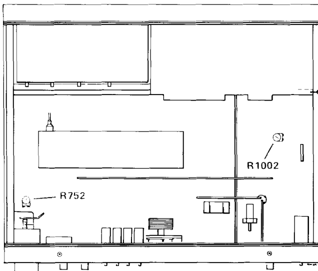
Figure 44 Test points
