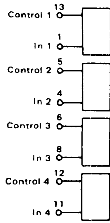
U501/502/601/907/908 MC14066CP
