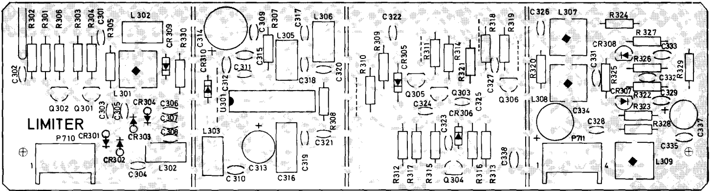
Figure 18 Limiter/detector board below serial No. 00700, component side
