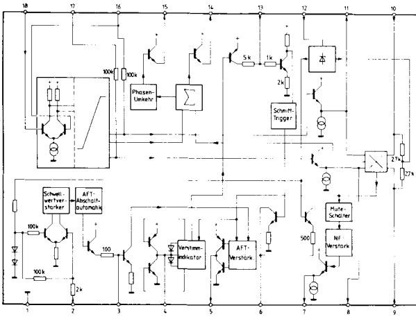
U301 TDA1047
