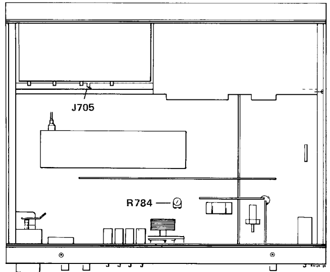
Figure 11 Dial pointer adjustment
