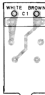
Figure 58 Power switch board, component side
