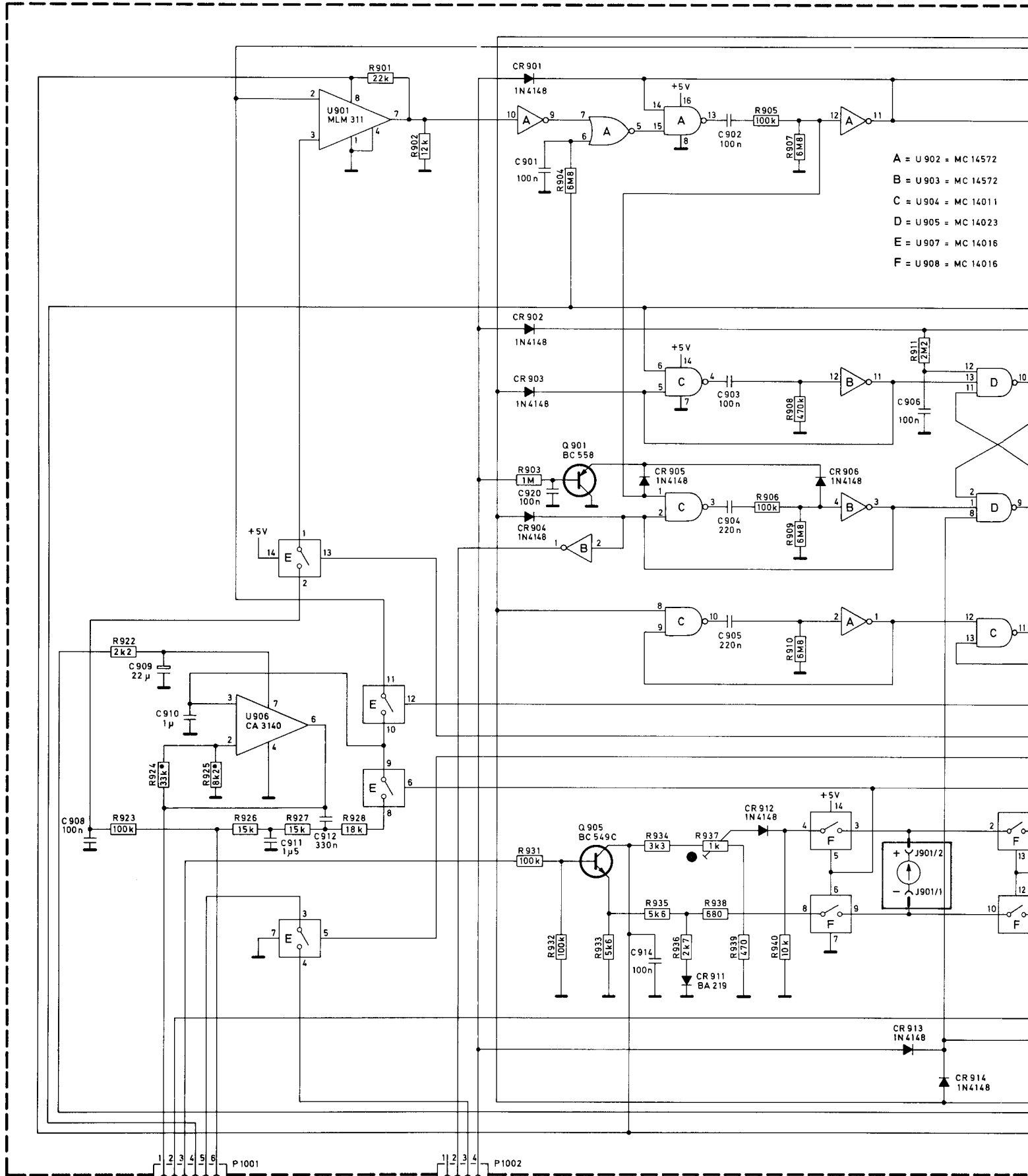
Figure 41 Tuning system 1
