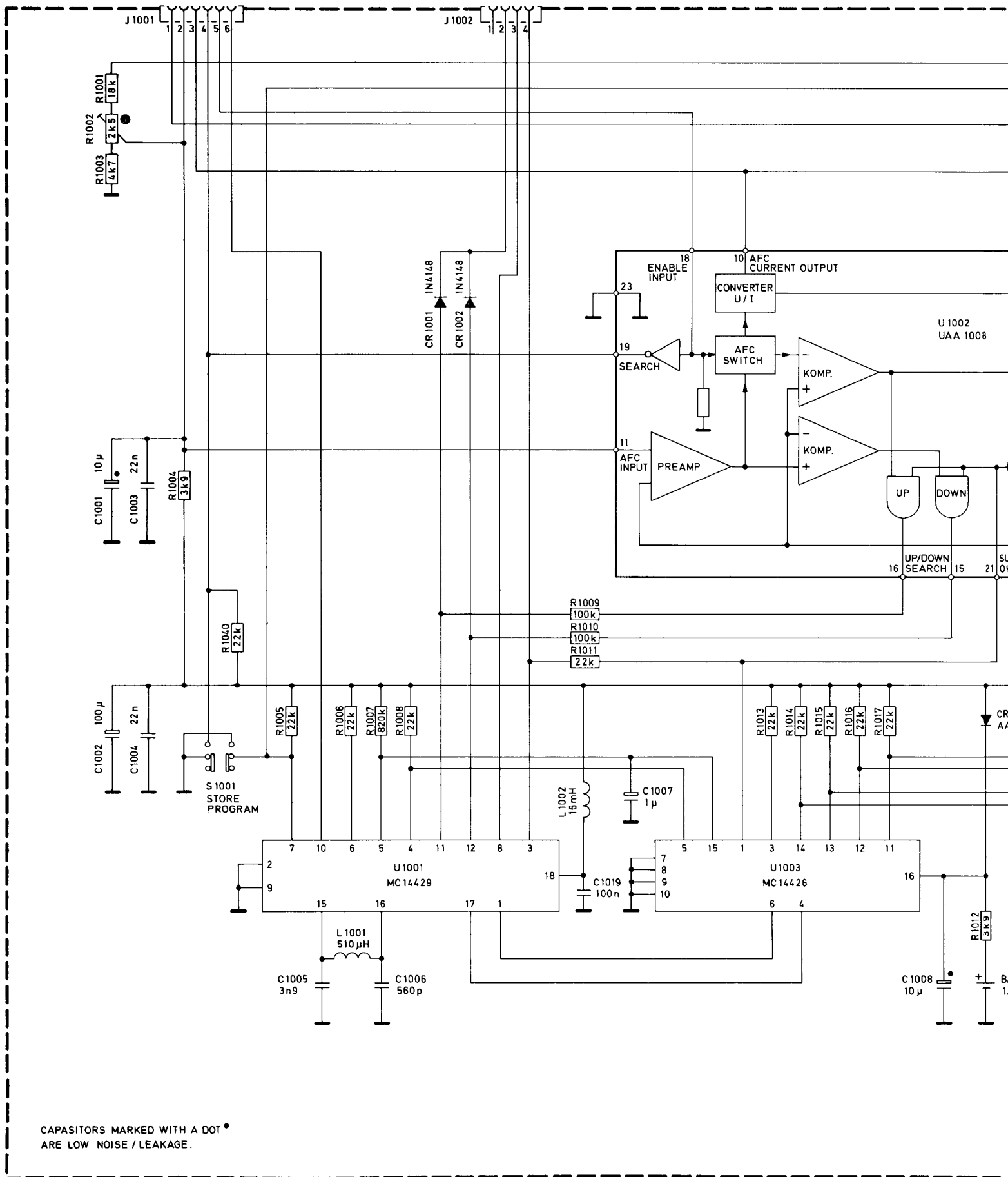
Figure 45 Tuning system 2
