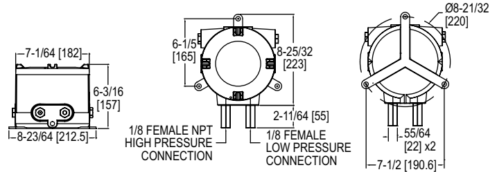
AT-102NA-3000MR/MRS, shown with VS0 port/valve configuration
