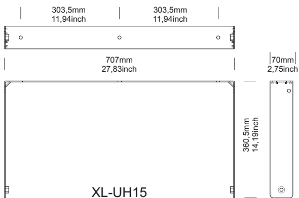
Wall metal bracket to mount in horizontal position
