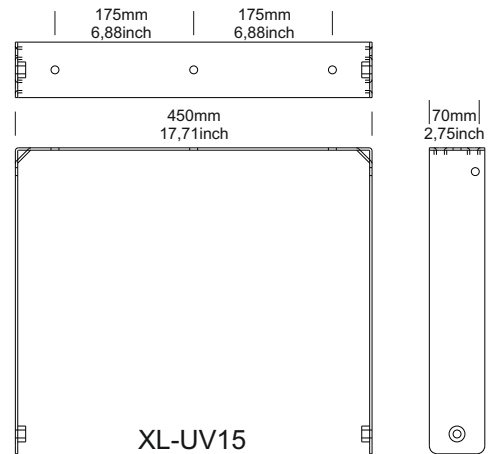
Wall metal bracket to mount in vertical position
