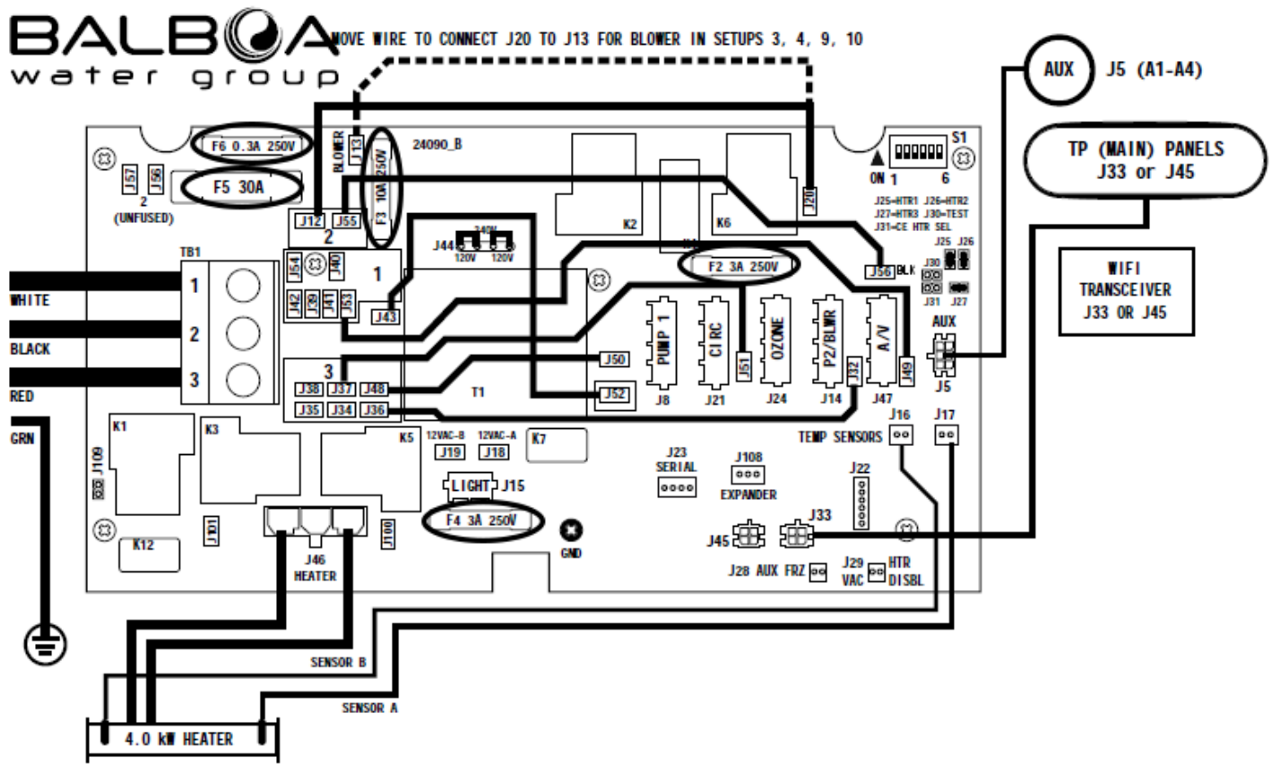
“Typisk panel-layout”
