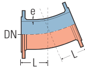
double 22.5° (1/16) flanged bend
