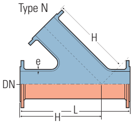
45° angle branch
