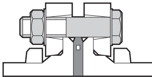
Adjustable flange
