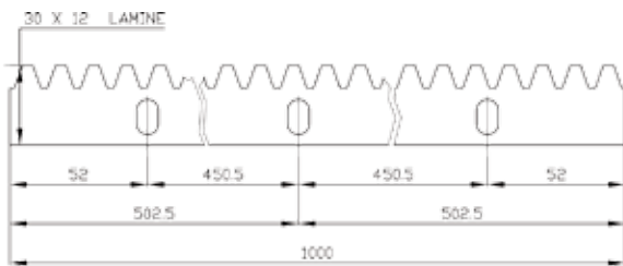
MODULE m=4 ANGLE OF PRESSION \alpha = 20^\circ
