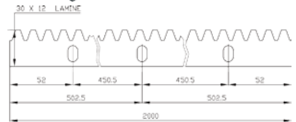
MODULE m=4 ANGLE OF PRESSION \alpha = 20^\circ
