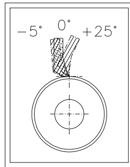
Inclinazione lama Knife inclination while working
