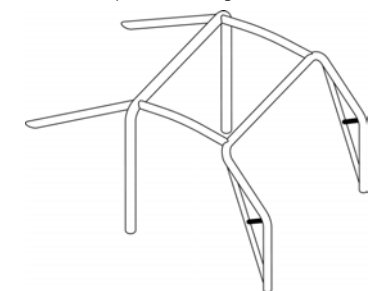
Dessin/Drawing 253-33
