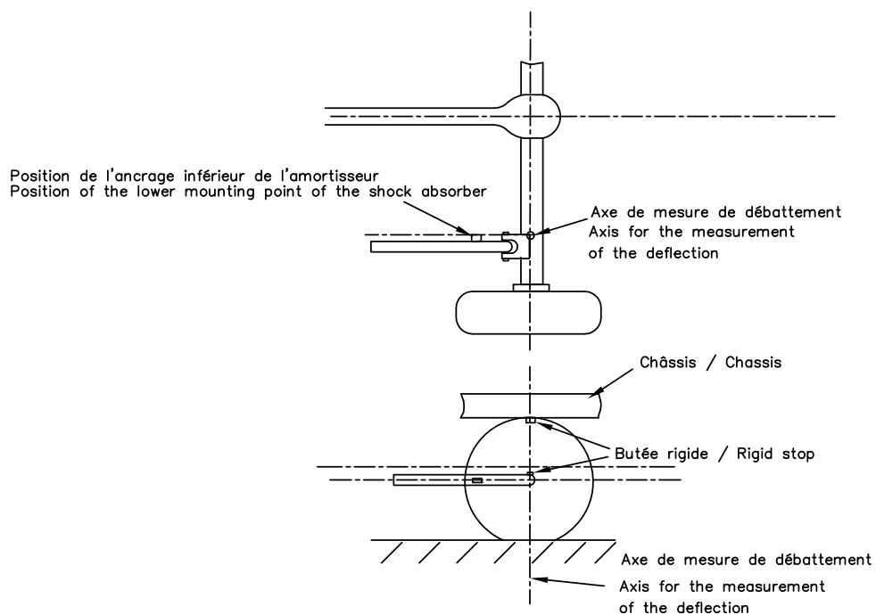
Dessin/Drawing 285-1
