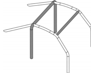
Dessin/Drawing 253-3
