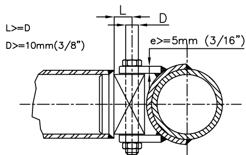
Dessin/Drawing 253-40
