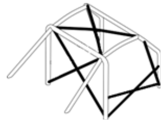
Dessin/Drawing 253-36
