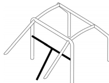
Dessin/Drawing 253-27
