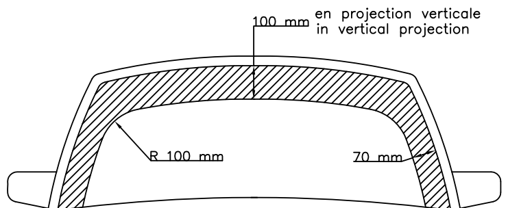
Dessin/Drawing 253-48
