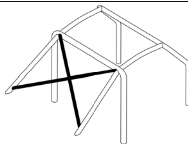
Dessin/Drawing 253-21
