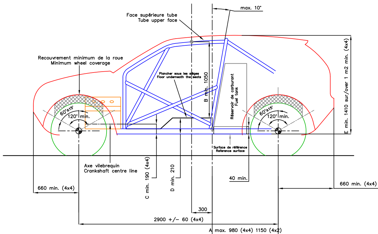
Dessin/Drawing 285-1
