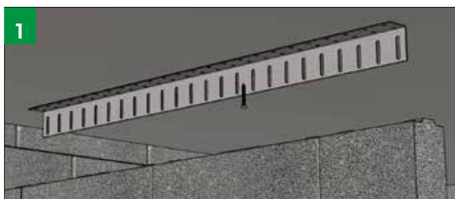
1 Montera takprofilen i taket.
