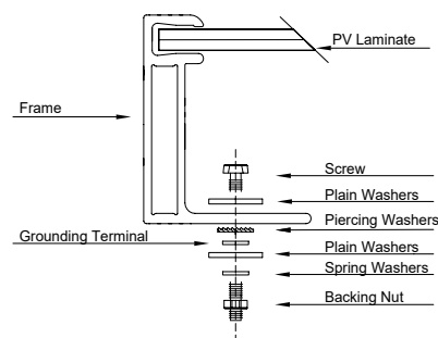
Figure 10: Grounding screw assembly detail
