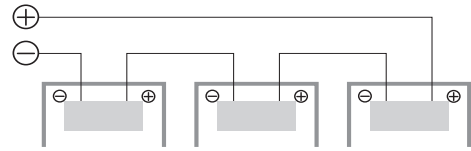
Series Wiring (Voltage Additive)
