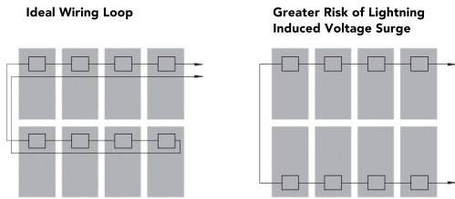
Figure 5: Wire loop design recommendation
