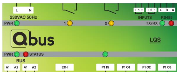
Figuur 7 LQS06SA Front detail LEDs
