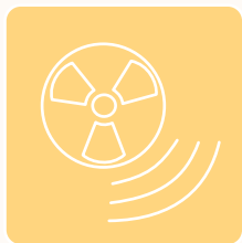
Ionising radiation
