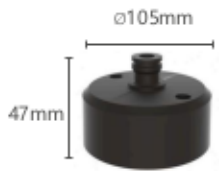
SB Surface Base Mount
