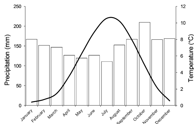
Fig. 2 Climate data from 1949 to 2007 at the Fagurhólsmýri weather station (data supplied by the Icelandic Meteorological Office). Mean monthly temperature (solid line), mean monthly precipitation (bars)
