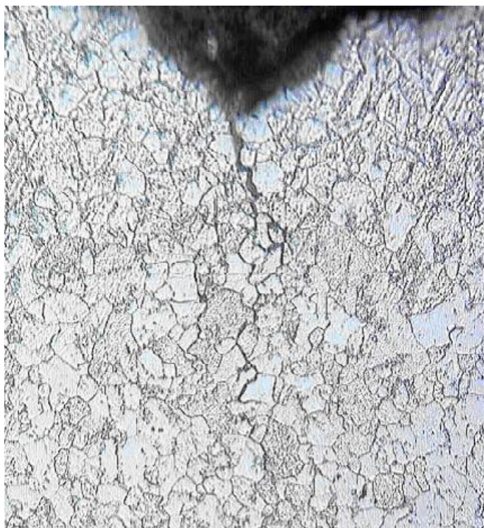
Figure 4-148 – Photomicrograph of a crack in the tube shown in Figure 4-147.
