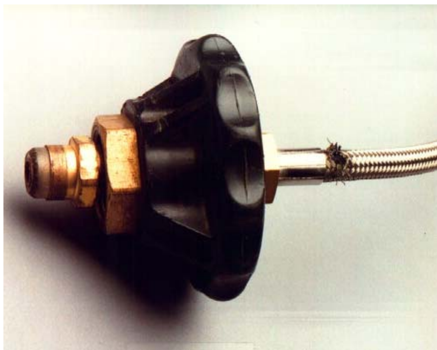
Figure 4-69 – Burnthrough of a PTFE-lined stainless steel hose in high pressure gaseous oxygen (GOX) service. Grease contamination ignited and penetrated the hose.
