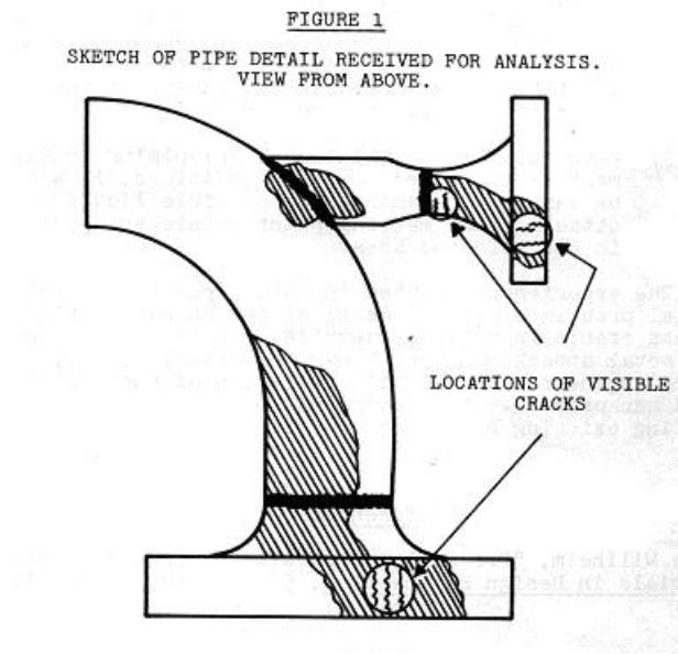
Figure 4-157 – Sketch of a stainless steel elbow that suffered liquid metal embrittlement as a result of dripping molten zinc during a fire.
