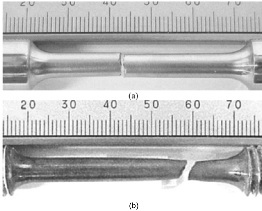
Figure 4-7 – Tensile tests from 304H stainless steel FCC flue gas line with 12% sigma phase. The top bar (a) failed in a brittle manner at room temperature The bottom sample (b) was tested at the operating temperature and shows significant ductility and elongation 1,320°F (716°C), Reference 6.
