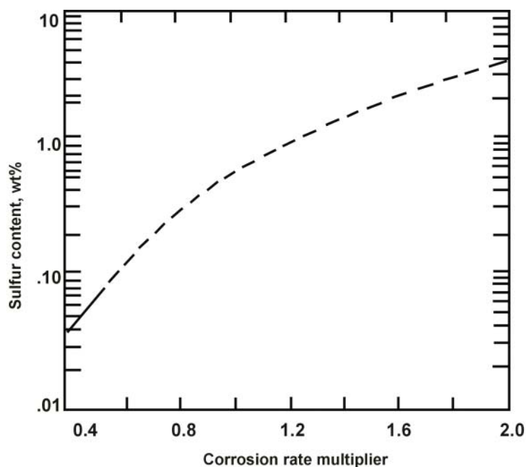
Figure 4-115 – Multiplier for corrosion rates in Figure 4-112 based on differing sulfur content of process fluid. (Reference 3)
