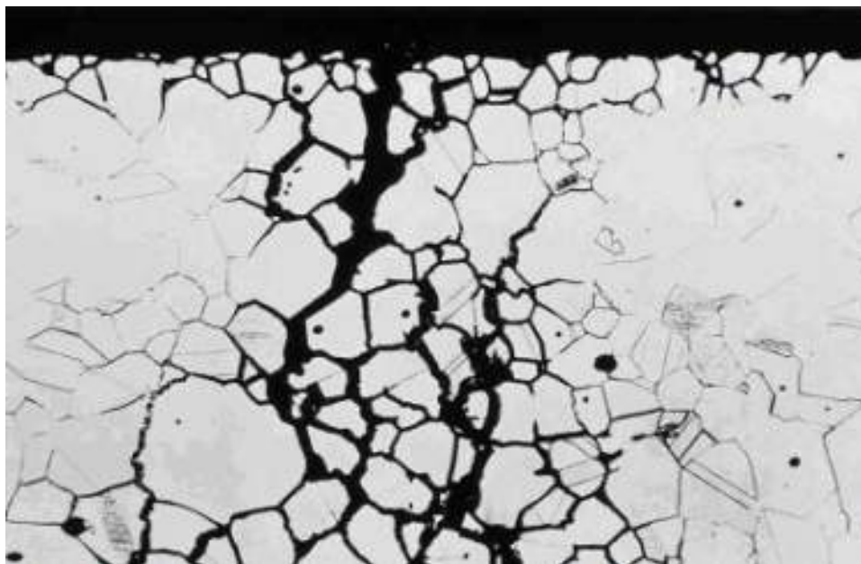
Figure 5-25 – High magnification photomicrograph of metallographic sample showing intergranular cracking and grain dropping.
