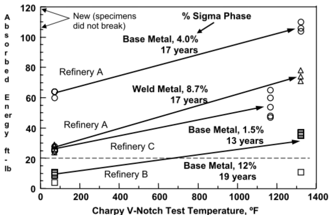
Figure 4-11 – Charpy V-Notch Impact Test Results as absorbed energy in ft-lbf, at room temperature and service temperature (Reference 6).
