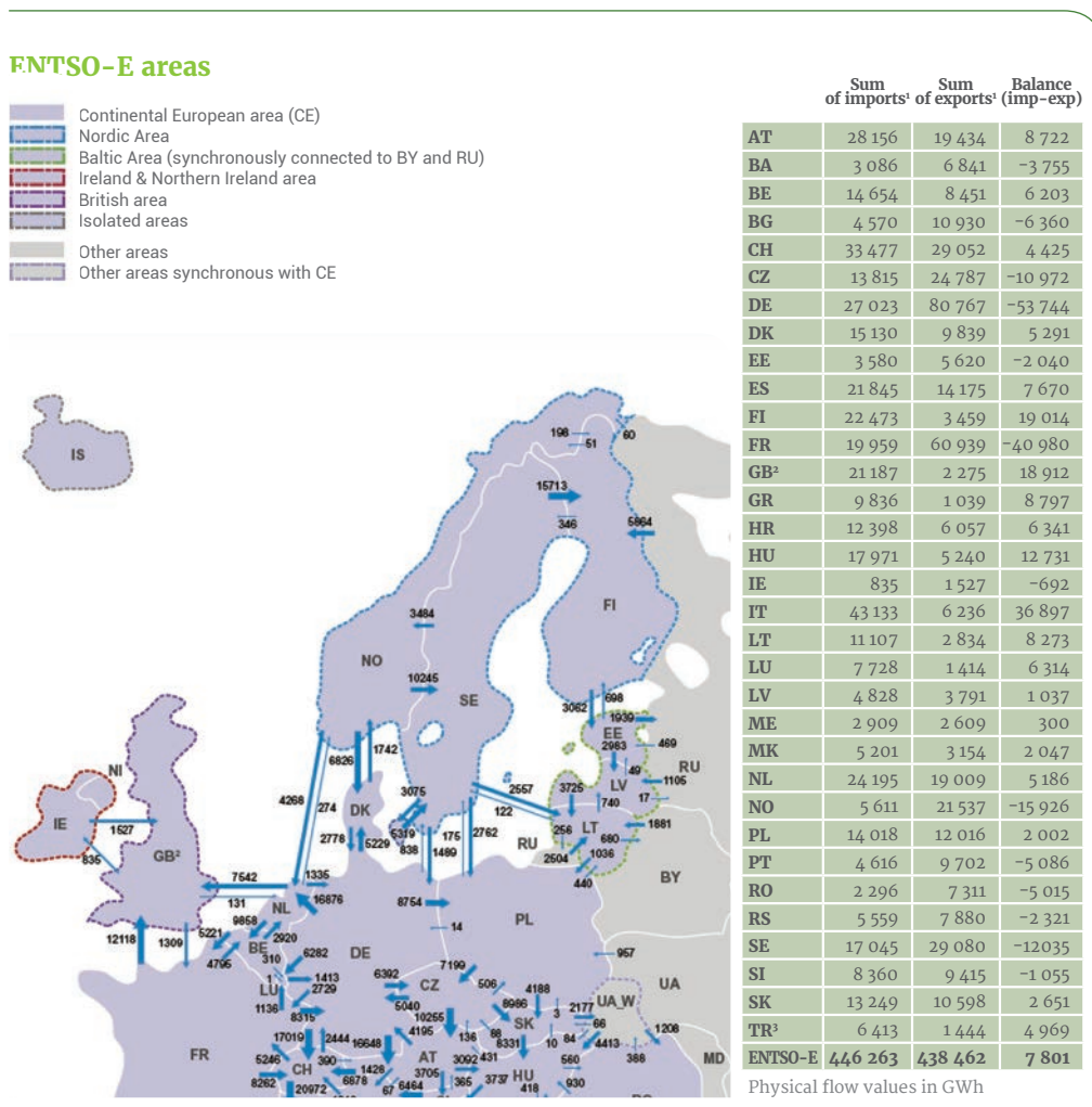
Figure 10 Cross border physical energy flows (GWh) in the Baltic Sea Region in year 2016 [Source: ENTSO-E]
