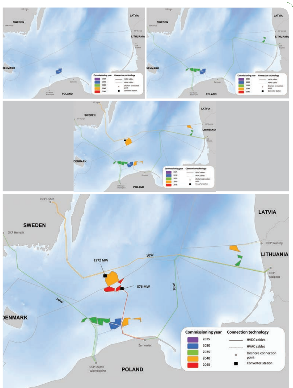
Figure 33 Case Study 1 – Scenario 1b schematic build-out
