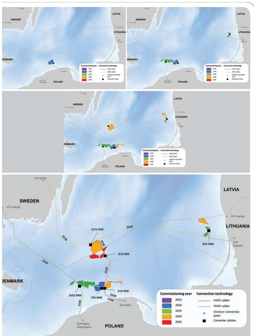
Figure 41 Case Study 1 – Scenario 3b schematic build-out
