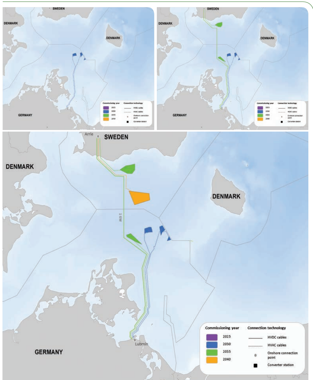
Figure 56 Case Study 2 – Scenario 1b schematic build-out
