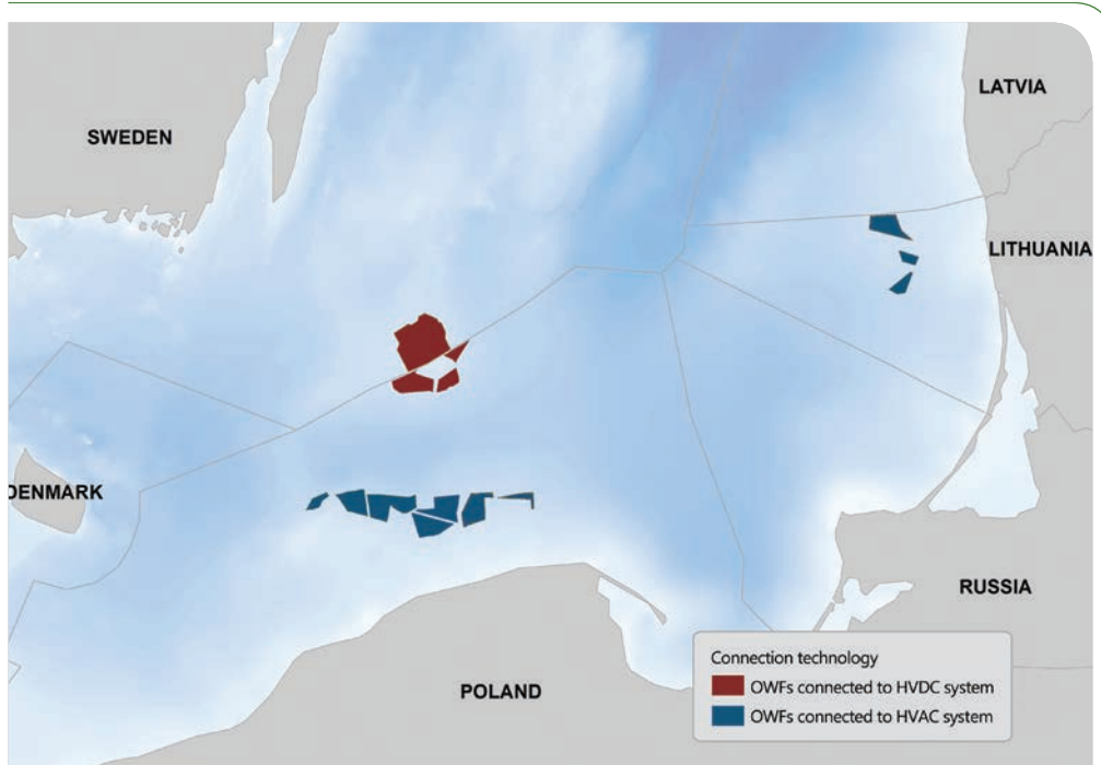
Figure 34 Case Study 1 – Scenario 1b OWF connection technology
