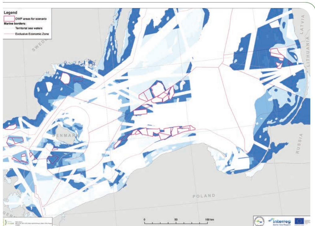
Figure 24 Map presenting constraints for offshore substations [Source: Baltic InteGrid project – Maritime Institute in Gdańsk]
