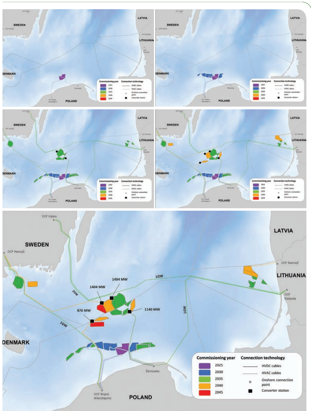
Figure 31 Case Study 1 – Scenario 1a schematic build-out
