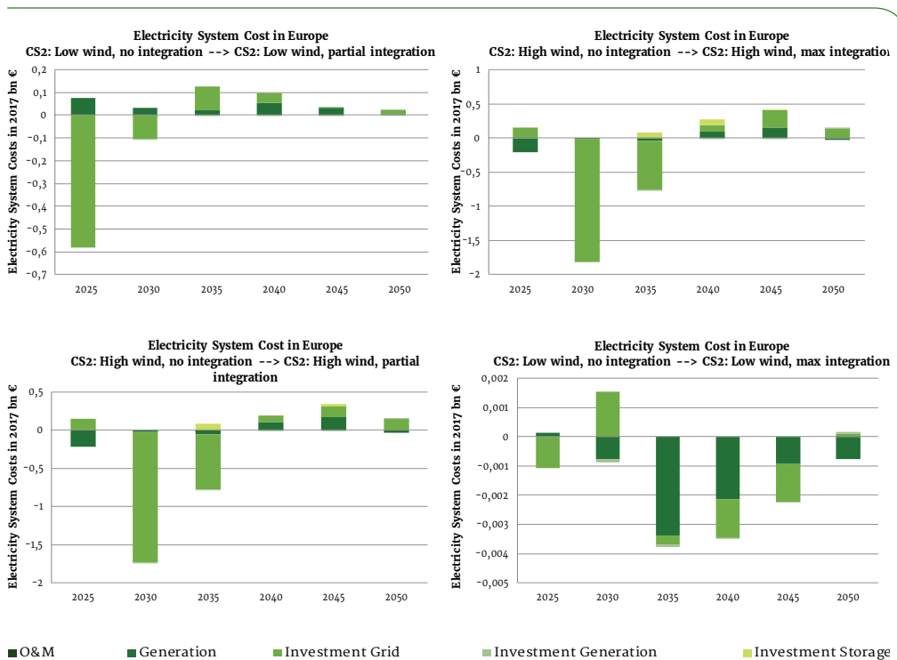
Figure 68 Electricity System Cost in Europe – Case Study 2
