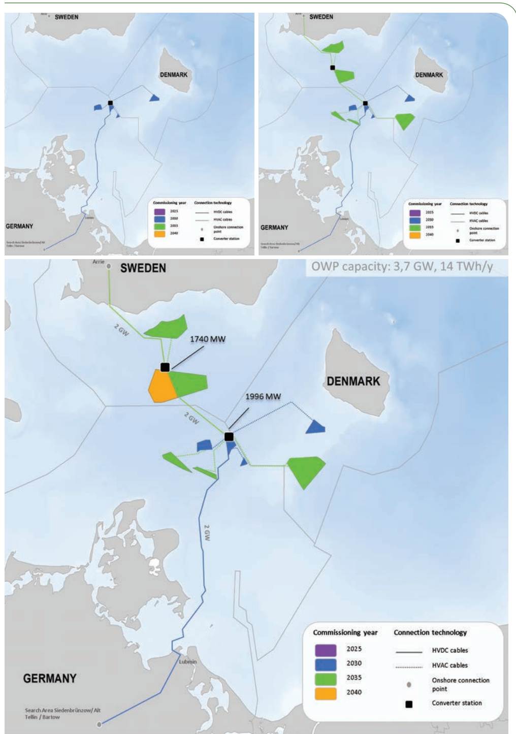
Figure 62 Case Study 2 – Scenario 3a schematic build-out
