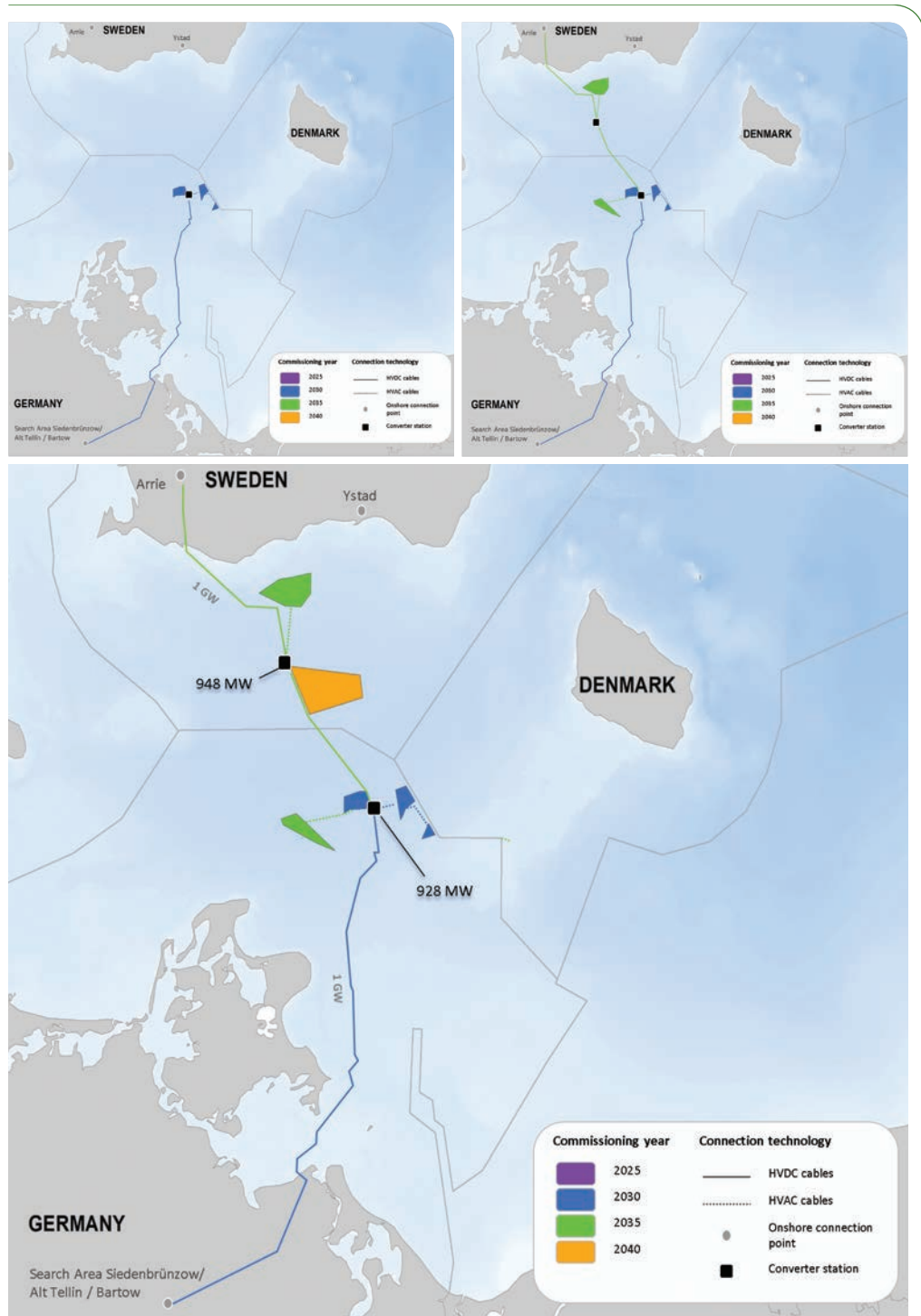
Figure 64 Case Study 2 – Scenario 3b schematic build-out
