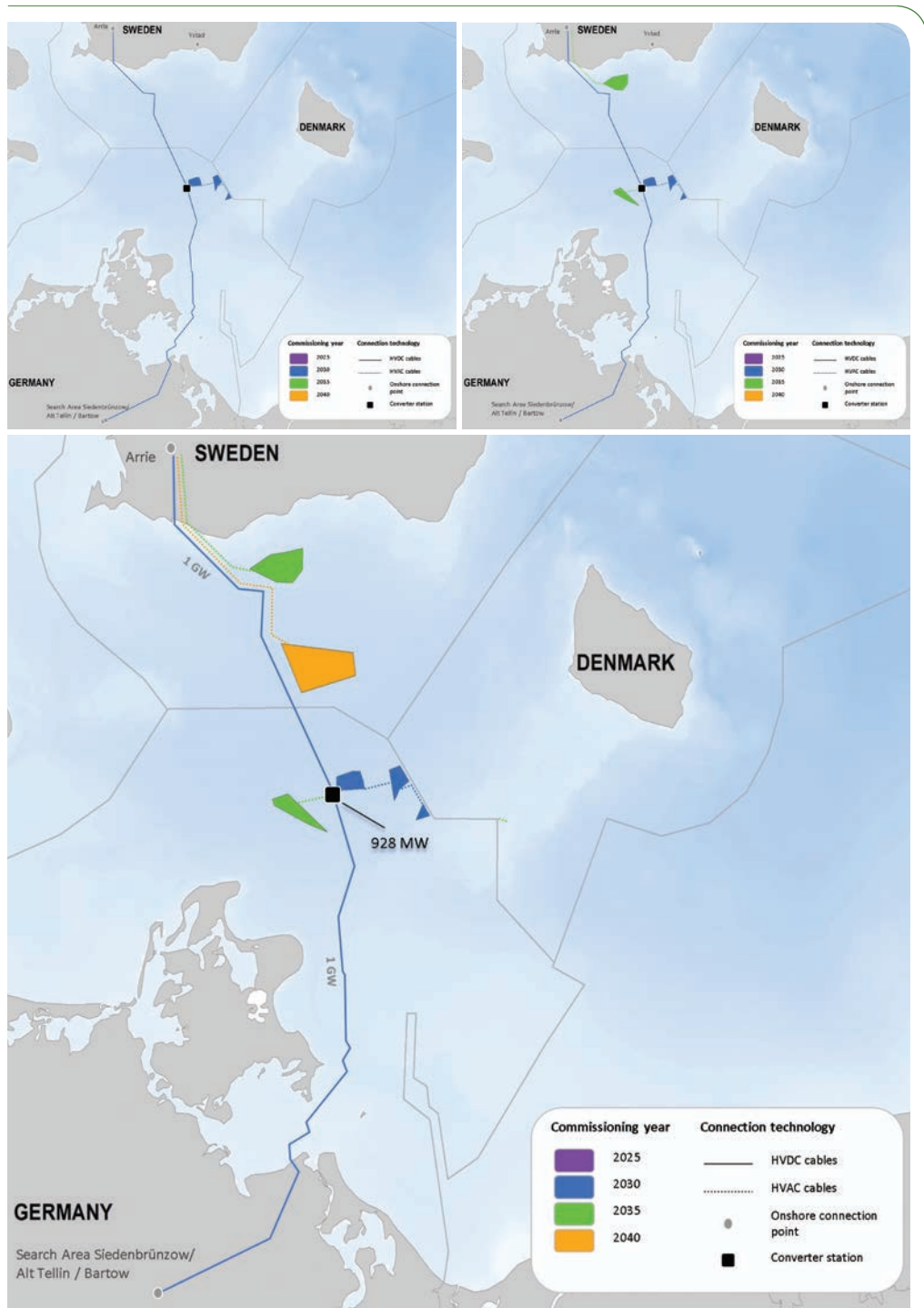
Figure 60 Case Study 2 – Scenario 2b schematic build-out
