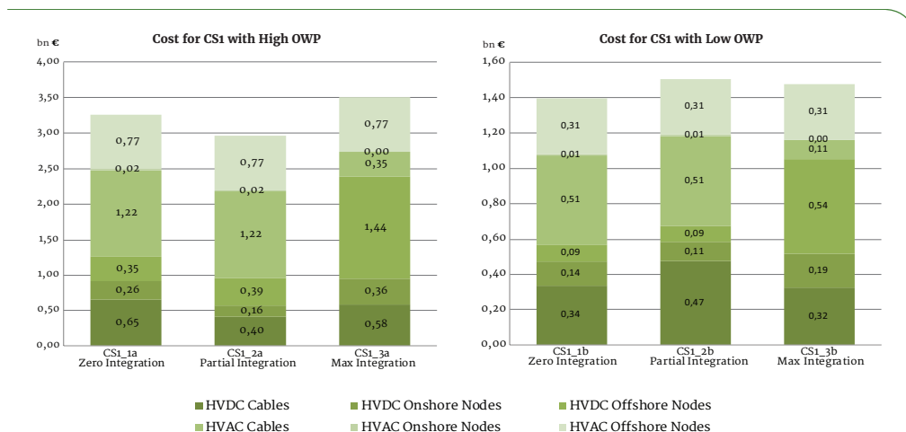
Figure 46 Cost structure for the scenarios in Case Study 1
