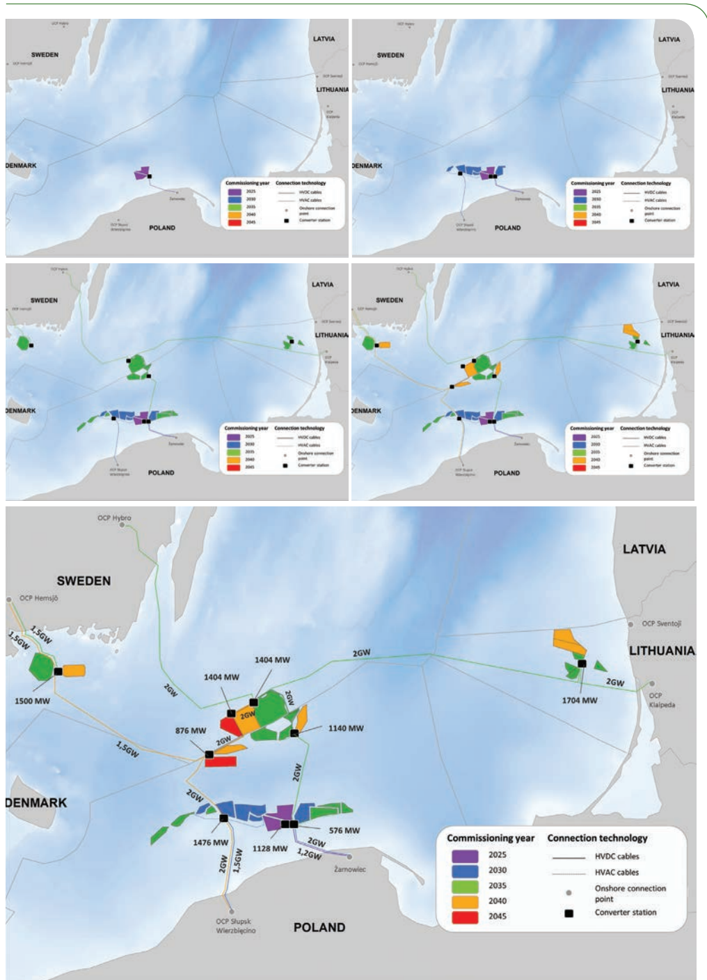
Figure 39 Case Study 1 – Scenario 3a schematic build-out
