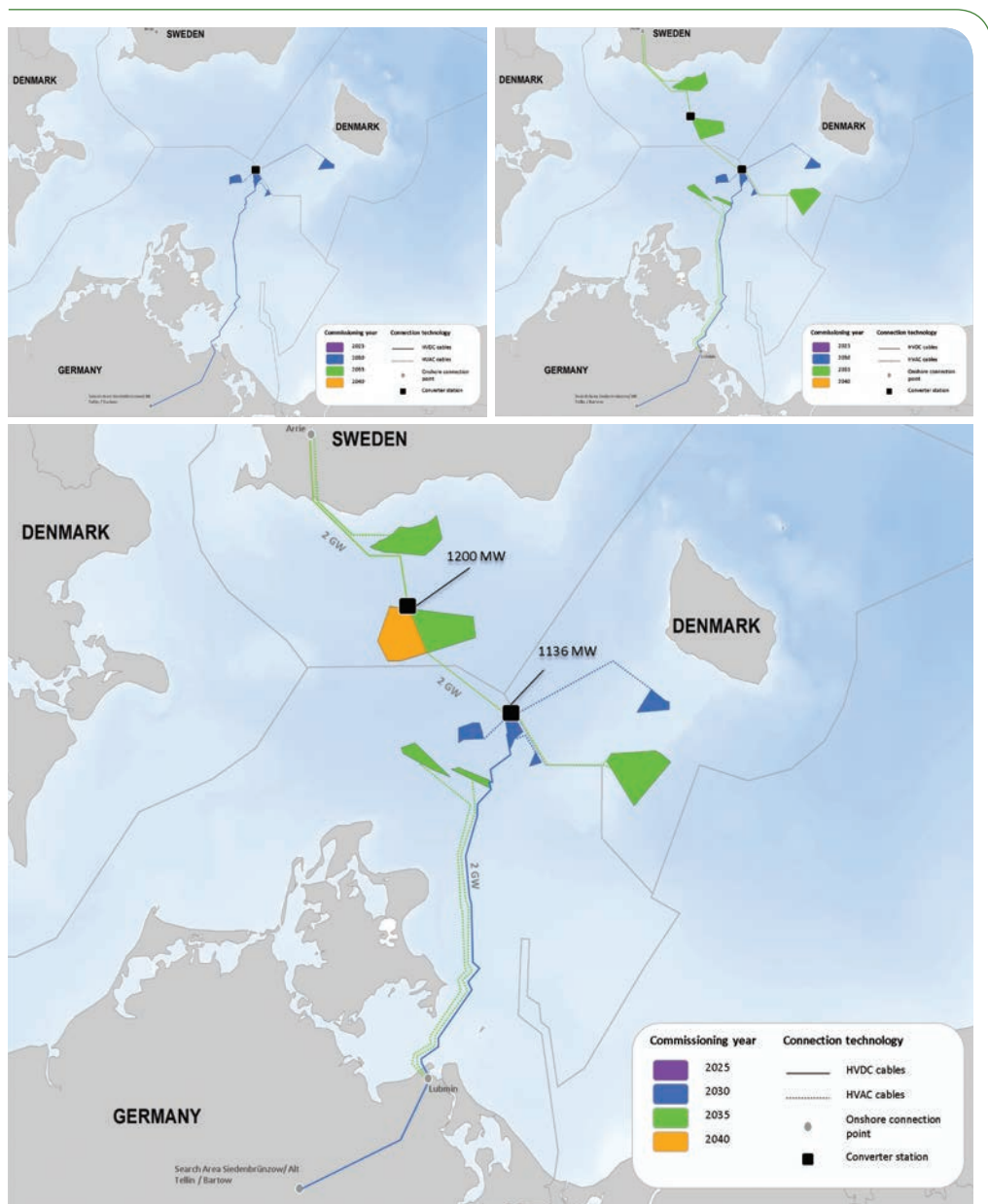
Figure 58 Case Study 2 – Scenario 2a schematic build-out
