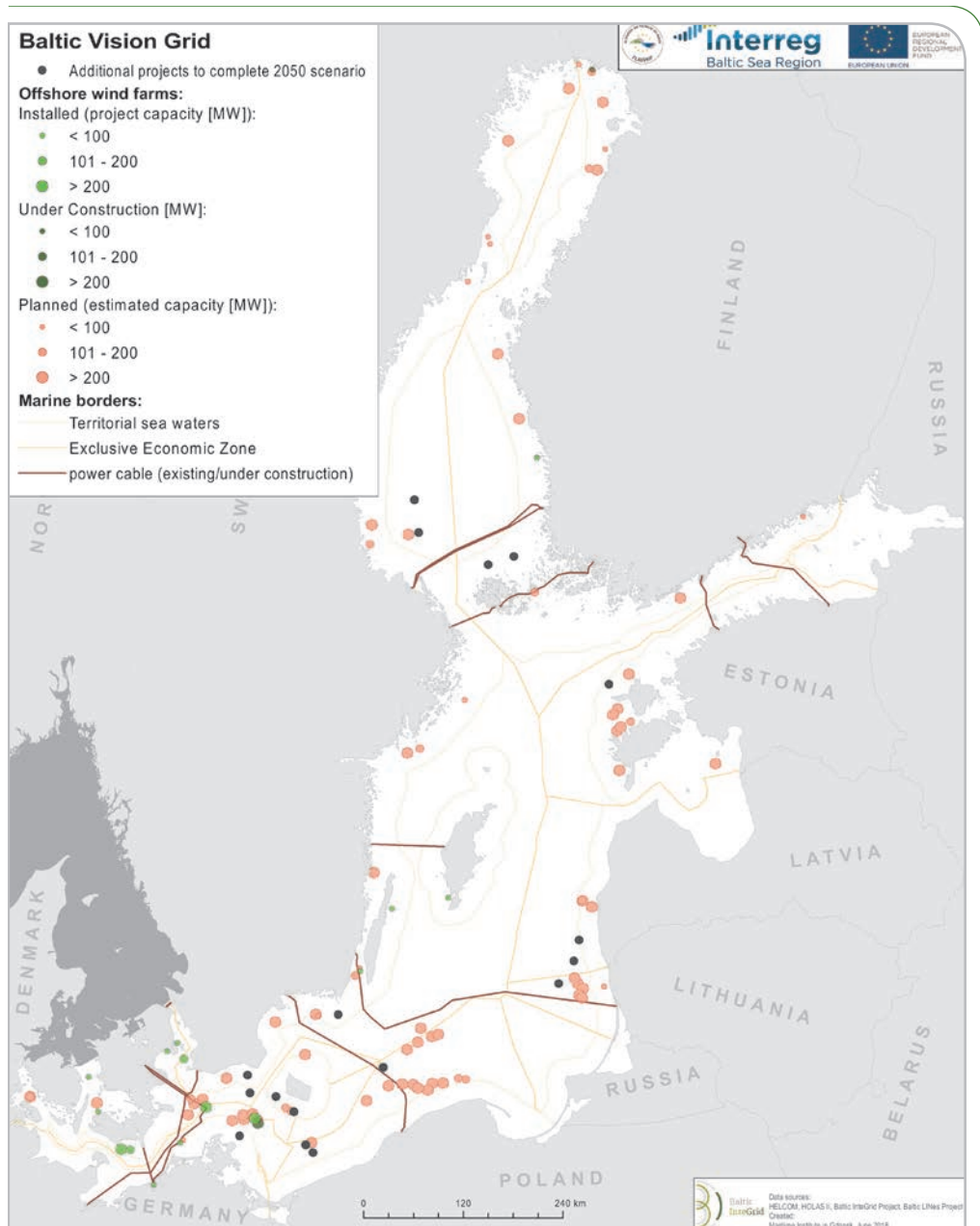
Figure 20 Map of existing and planned OWFs and interconnection projects in the Baltic Sea – status as of June 2018
