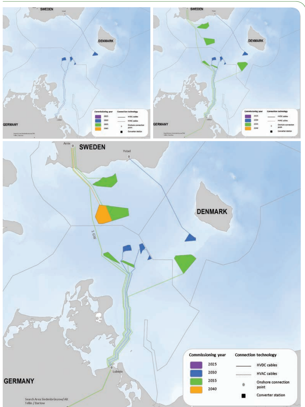
Figure 54 Case Study 2 – Scenario 1a schematic build-out
