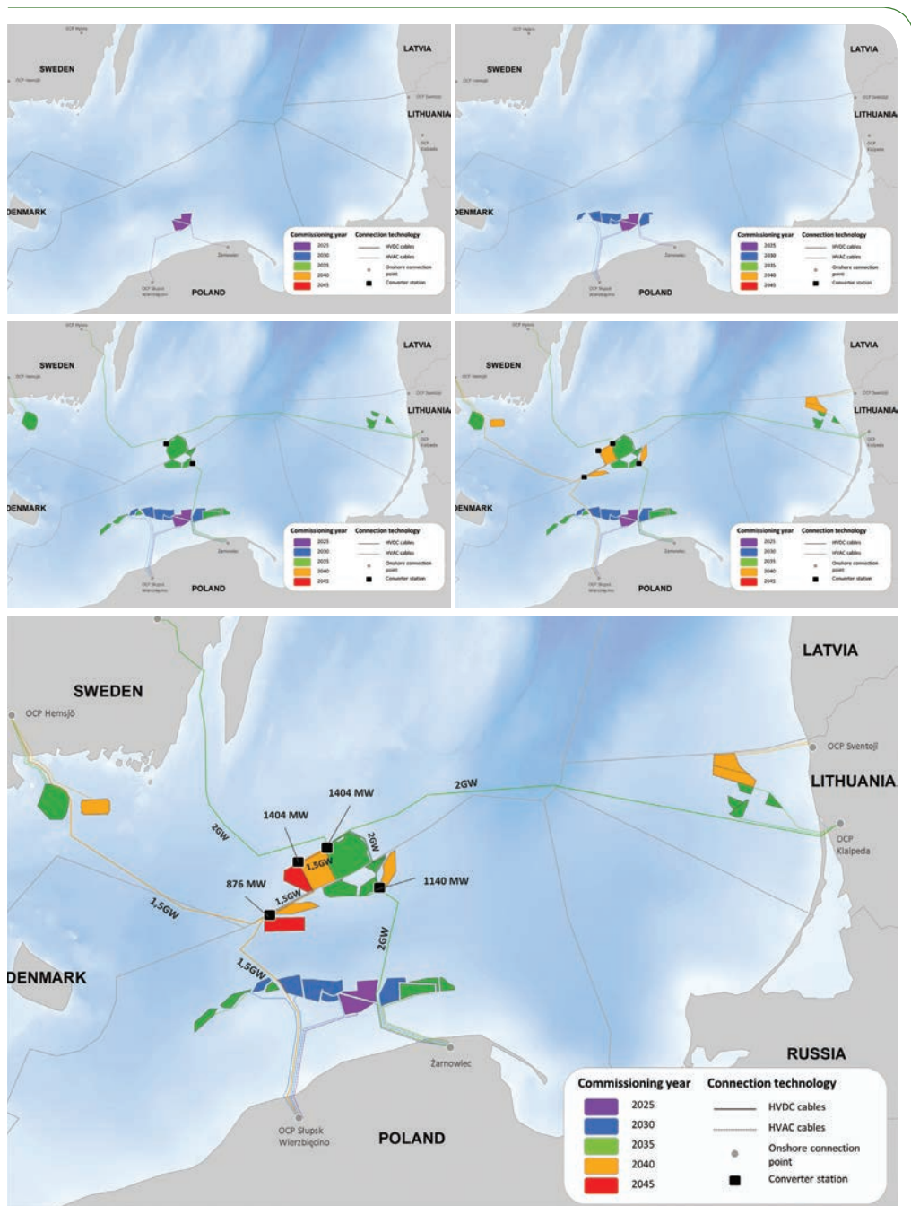
Figure 35 Case Study 1 – Scenario 2a schematic build-out
