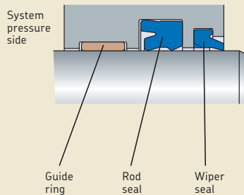
Typical rod seal arrangement for light to medium duty hydraulic applications
