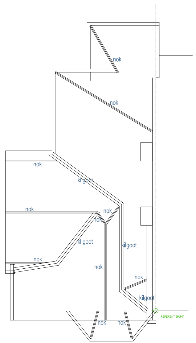
DAKPLAN
