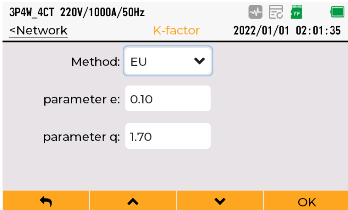
Figure 5-15 K-factor para setting
