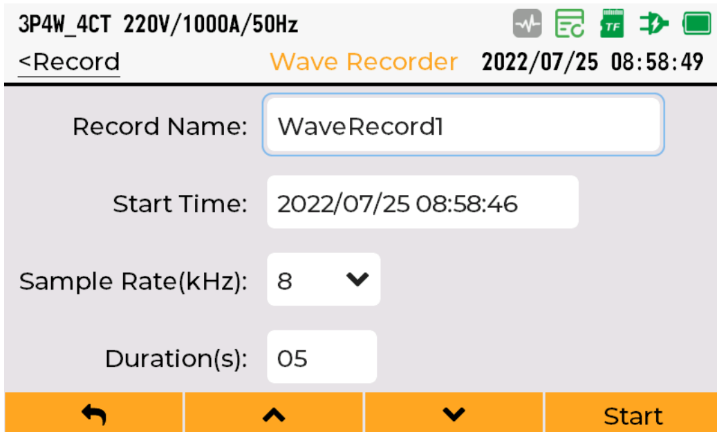
Figure 4-5 Waveform Recorder
