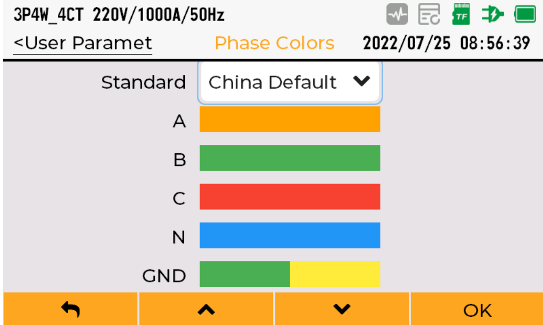
Figure 5-28 Phase sequence color setting
