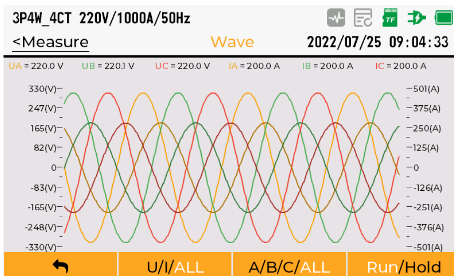
Figure 5-38 Voltage and current waveform display
