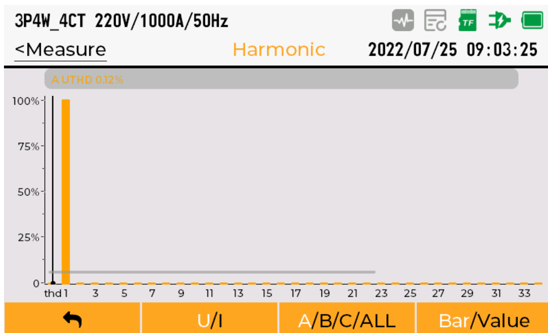
Figure 5-36 Harmonic histogram display
