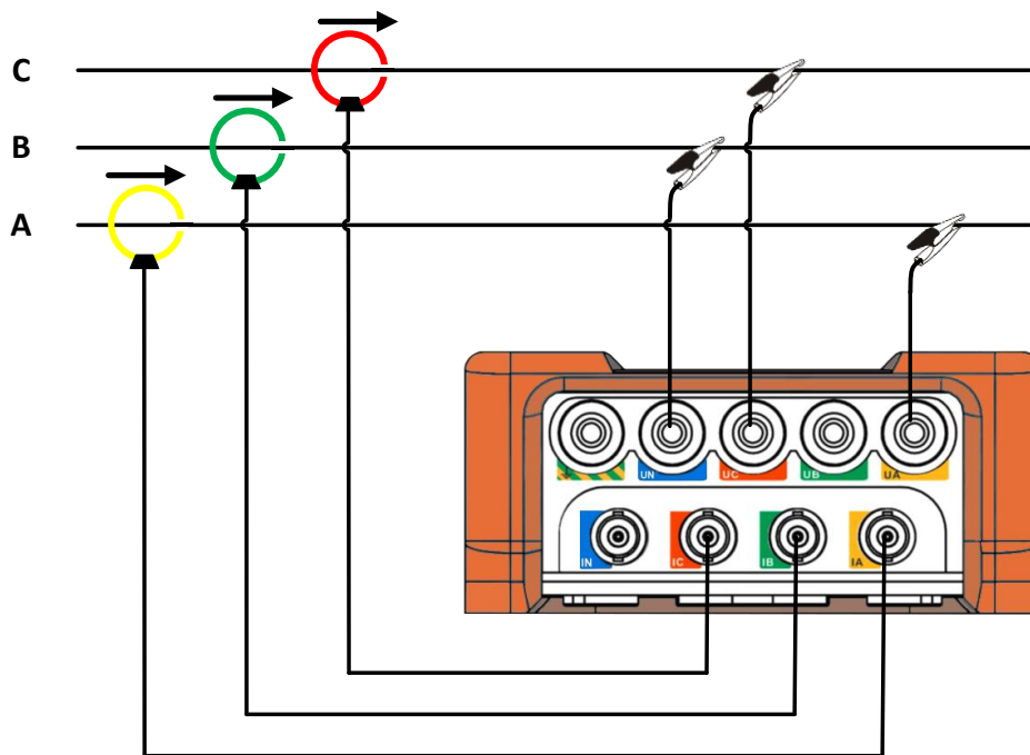
Figure 3-3 3P3W_3CT
