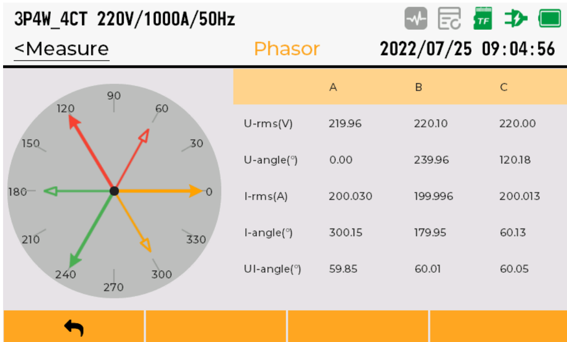
Figure 5-40 Vector diagram display
