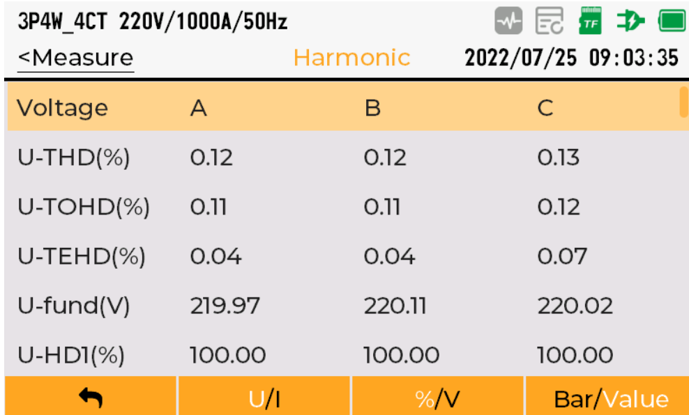
Figure 5-37 Harmonic value display
