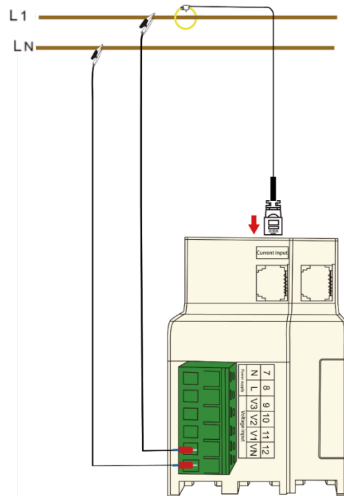
One phase and two-wire
