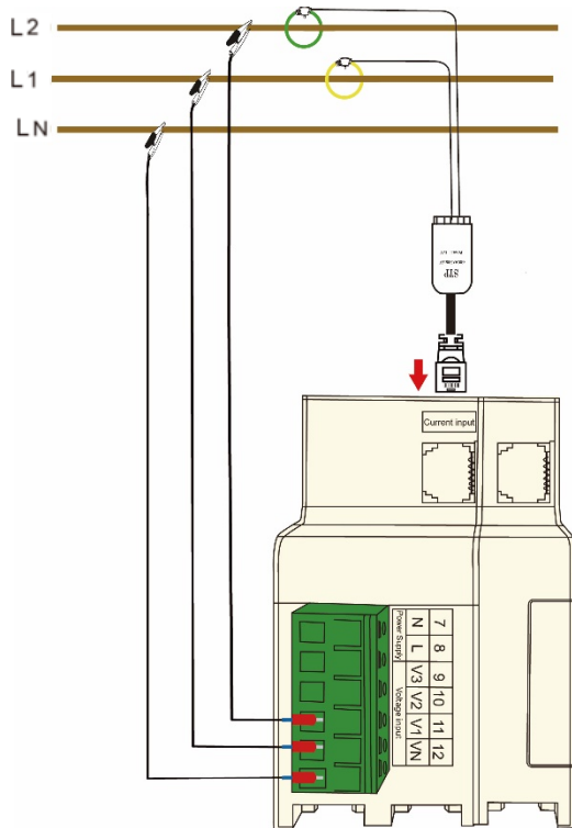
One-phase three-wire
