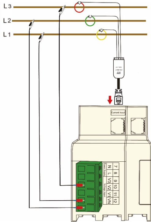
Three-phase three-wire 3CT
