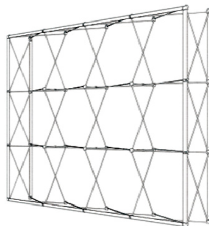
3x4 modul - 297x224x36 cm (BxHxD)
