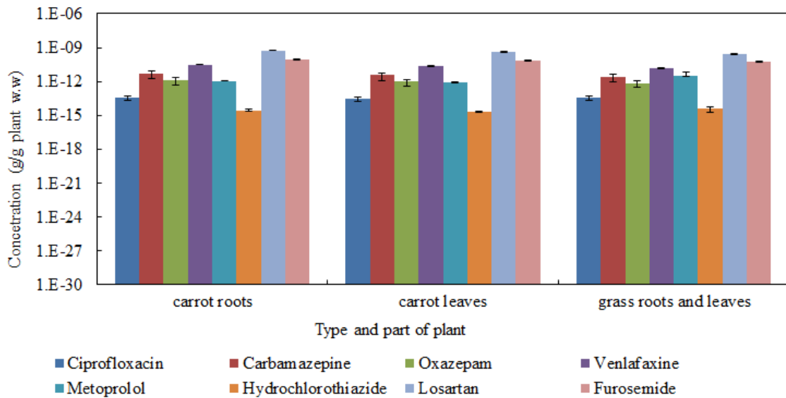
Figure 16. The average concentrations (g/g ww) of selected pharmaceuticals in the roots and leaves of carrot and grass plants after 100 days in the growing season during the first, second and third year of blackwater fertilization with blackwater after liquid composting and ammonia treatment (40 ton/ ha. year), simulated using BASL4 model. The bars show standard deviations.
