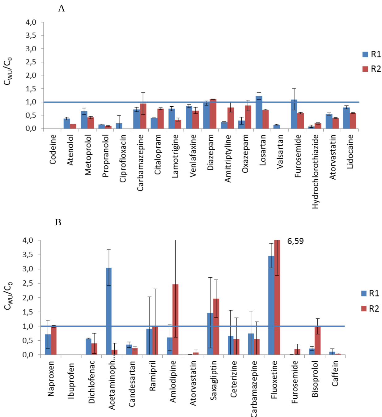
Figure 8. Changes of pharmaceutical concentrations in blackwater treatment ( n=2 ): reactor R1 and R2 after liquid composting and ammonia treatment for A) substances analyzed at SLU, and B) substances analyzed at SPPD. Values above 1 indicate an increase in concentration during treatment and below 1 indicate a reduction in concentration during treatment. Pharmaceuticals "evolution" during treatment was calculated as C_{treated\ BW}/C_0 . "C" is expressed in ng/L and is the sum between the concentrations detected in the solid and liquid phase.
