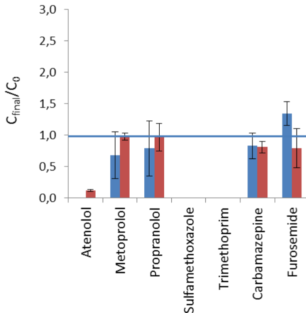
Figure 7. Changes of concentrations of spiked pharmaceuticals in fecal sludge ( n=2 ) after mesophilic (+37 °C, 61 days, blue bars) and thermophilic (+52 °C, 59 days, red bars) anaerobic treatment. Values above 1 indicate an increase in concentration during treatment and below 1 indicate a reduction in concentration during treatment. The change of pharmaceutical concentration during treatment was calculated as C_{61d}/C_0 for mesophilic, and as C_{59d}/C_0 for thermophilic. "C" is expressed in ng/L and is the sum between the amounts detected in the solid and liquid phase.
