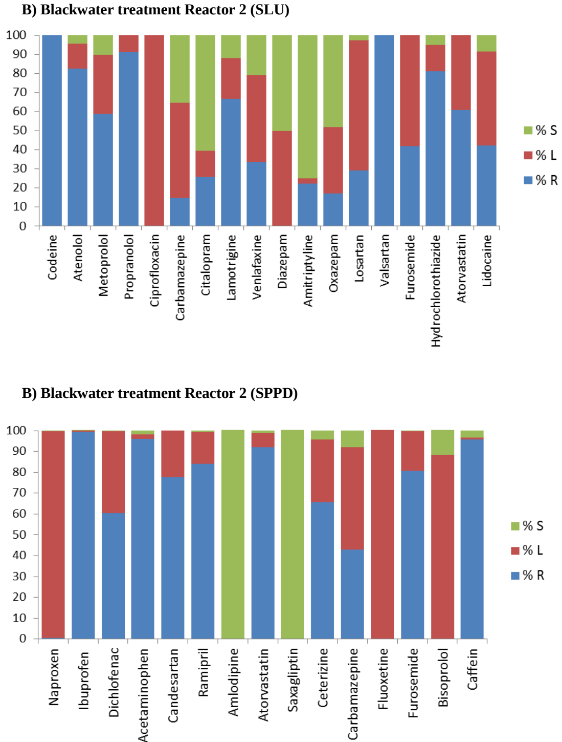
Figure 12 B. Percentage of pharmaceuticals removed (blue) during blackwater treatment (including liquid composting and ammonia treatment) and distribution of pharmaceuticals between the liquid phase (red) and solid phase (green) at the end of the treatment (%S: fraction of pharmaceutical remaining in the solid phase after treatment; %L: fraction of pharmaceutical remaining in the liquid phase after treatment; %R: percentage of pharmaceutical removed during treatment).
