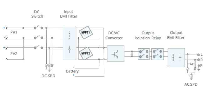
Circuit Diagram
