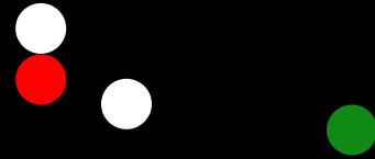
PILOT VESSEL ON DUTY STARBOARD SIDE (PILOTS HAVE A WHITE HAT & RED NOSE)
