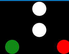
POWER DRIVEN VESSEL FROM AHEAD PROBABLY OVER 50 METRES
