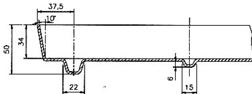
A-A (1/2)
