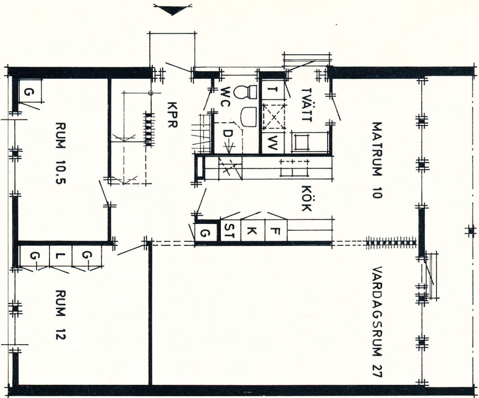
BOTTENPLAN
