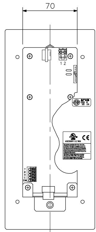
Rear View
