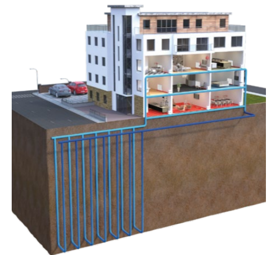
Figure 24 - Installation of the heating of the drilling Source: https://phpdonline.co.uk/features/ground-source-heat-pump-flats/
