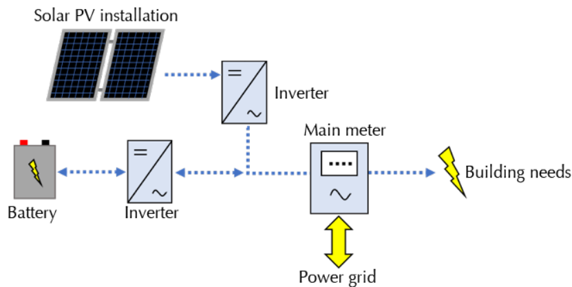
Figure 13 - Outline of an installation providing the local generation of electricity and energy storage.
