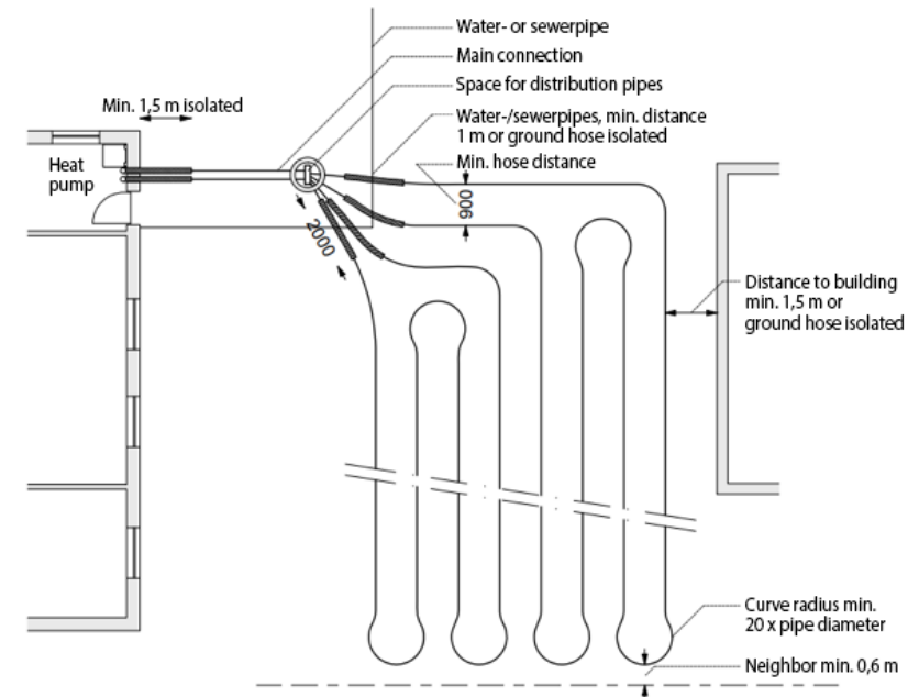
Figure 26 - Plan for locating ground hoses for horizontal installations [5]
