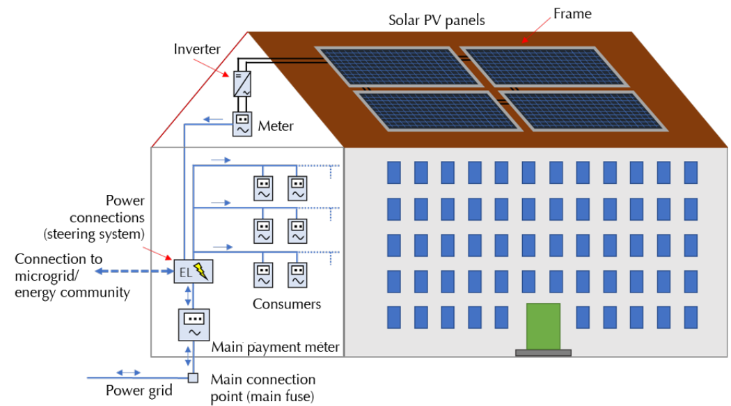
Figure 4 - Conceptual design of a PV installation in a energy community
