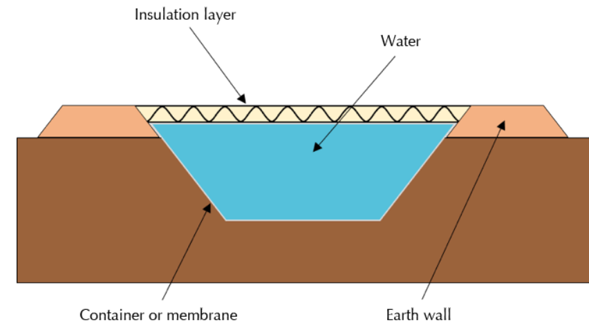
Figure 37 - Outline of a heat storage pond
