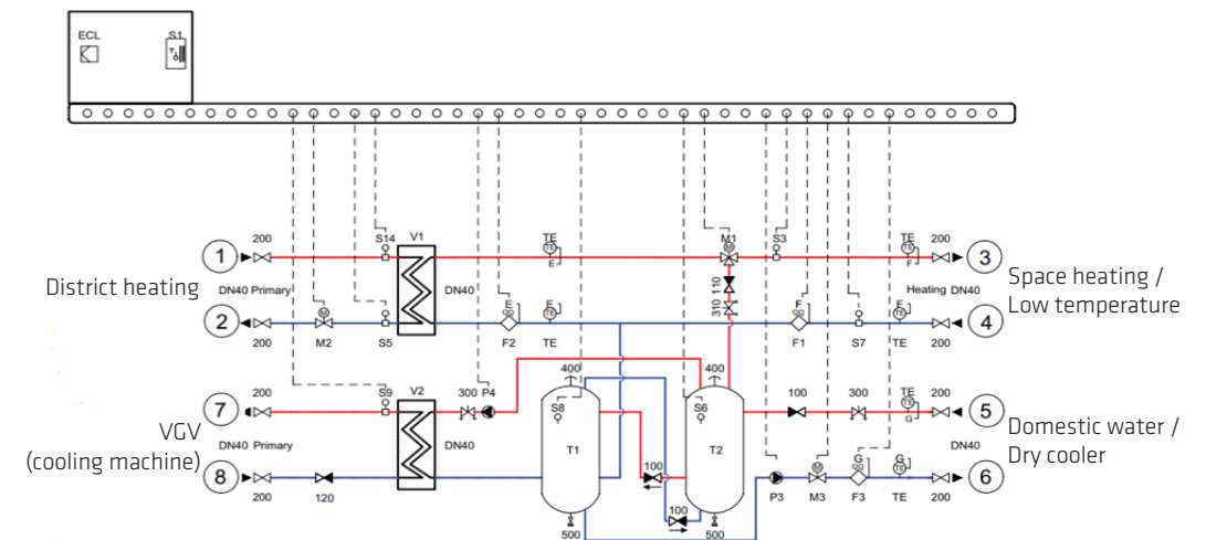
Figure 51 - Principle of a Danfoss heat recovery unit (HRU) with indirect connection to the district heating [2]
