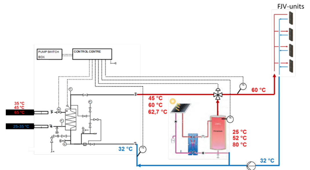
Figure 57 - Principle of a solar thermal installation in combination with district heating and installation of district heating units (Source: Alfa Laval)
