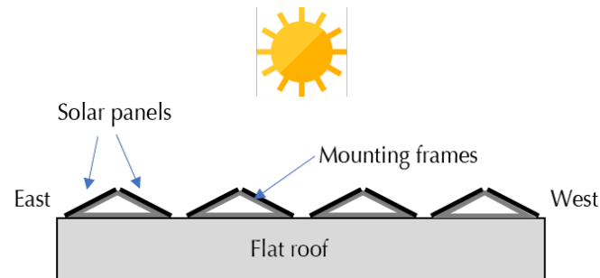
Figure 8 - Solar PV installations on a flat roof turning east-west, with double orientation
