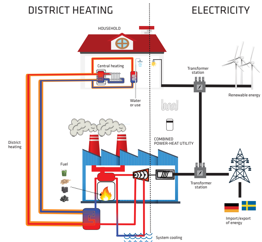
Figure 2: The Danish supply model based on cogeneration heat and power utilities, distribution companies and customers (in case shown as a single-family house, but could as well have been a tenant building or a larger company)
