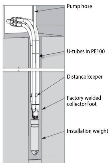
Figure 27 - Principle drawing of heat-drilling (from Rotek A/S) [1]. Energy collectors are made as double U-tubes.
