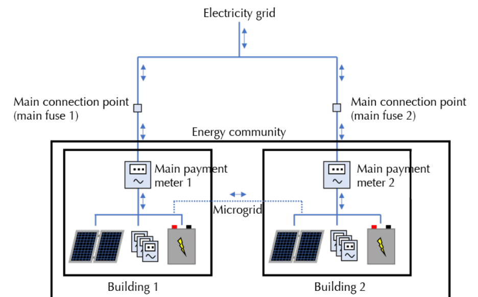
Figure 3 - Outline of the electricity grid with multiple buildings in the Energy Community
