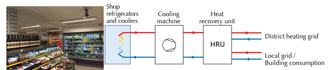
Figure 48 - Outline of a heat recovery installation with a cooling machine and a heat recovery unit
