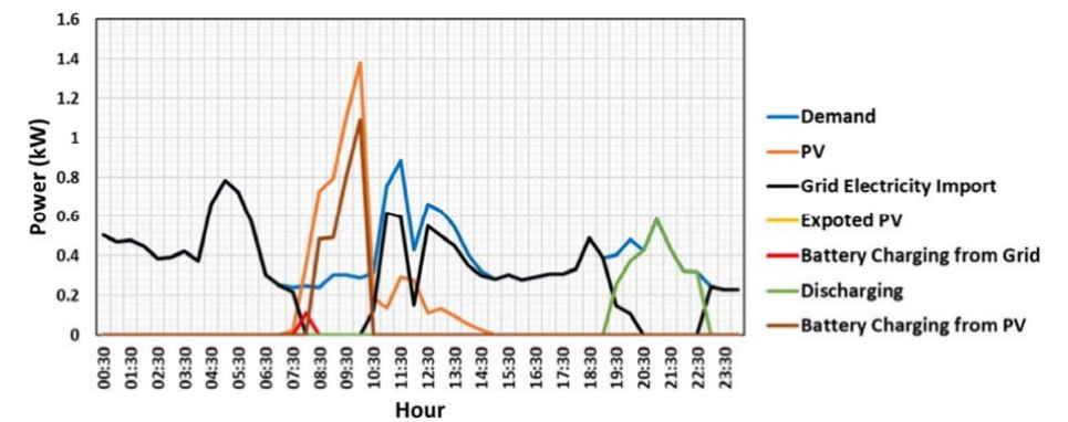
Figure 15 - Graph showing the ratio of power output from a photovoltaic installation integrated with a battery pack and energy use during winter (simulated) [4]
