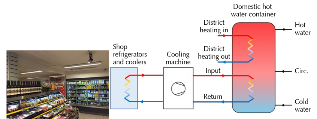
Figure 47 - Outline of a heat recovery installation with a cooling machine and a hot water container
