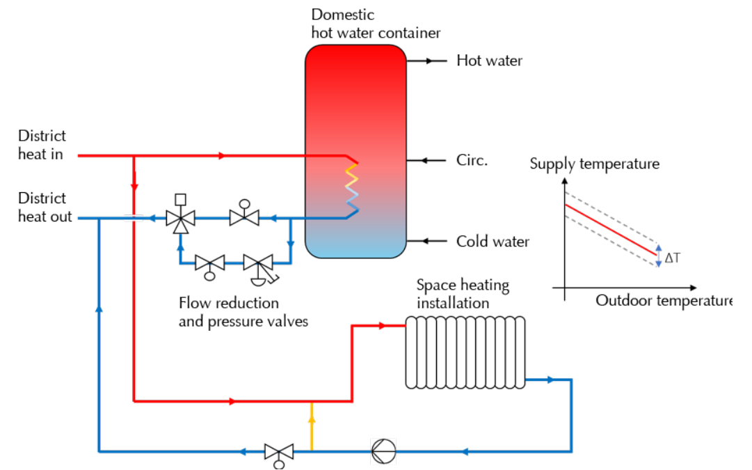
Figure 36 - Outline of space heating and hot water storage
