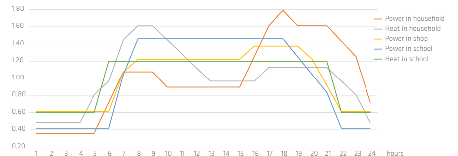
Figure 4: Day-based graphs (normalized) for typical household consumption of power and heat, as well as public institutions and shops consumption of power and heat showing peak load periods.
