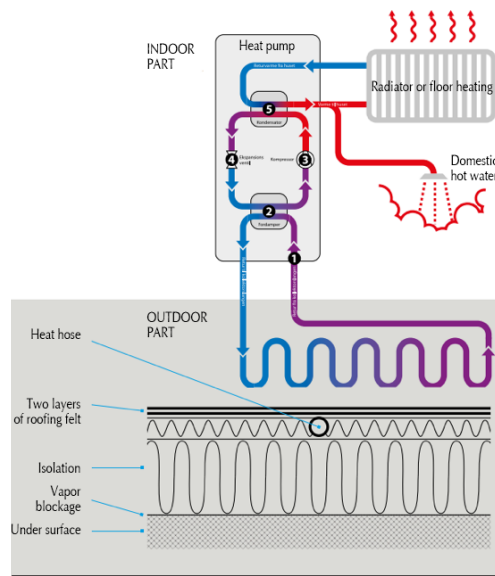
Roof installation
