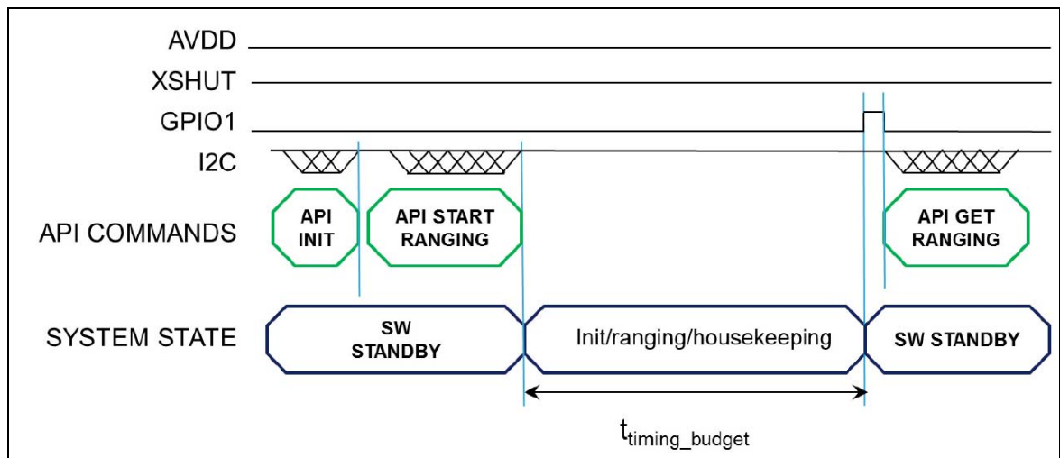
Figure 12. Ranging sequence
