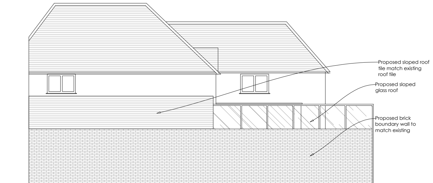
PROPOSED WEST SIDE ELEVATION
