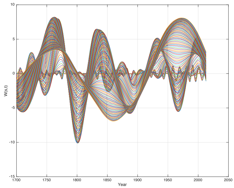
Figure 4: Wavelet spectrum W_h s(s, t) of the TSI-HS data series, for s = 1 \dots 190 .
