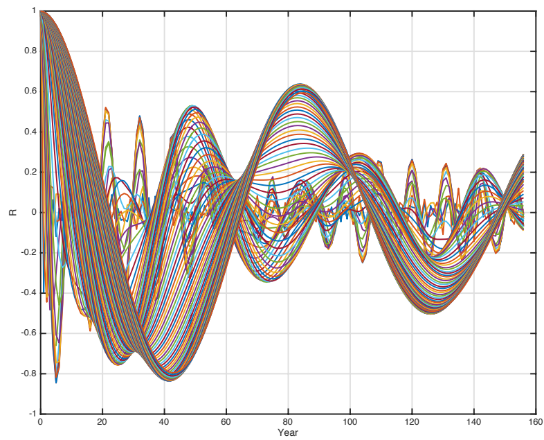
Figure 5: Autocorrelations Rhs(s, m) of the TSI-HS wavelet spectrum Whs(s, t) for s = 1 \dots 190 and m = 1 \dots 160 .
