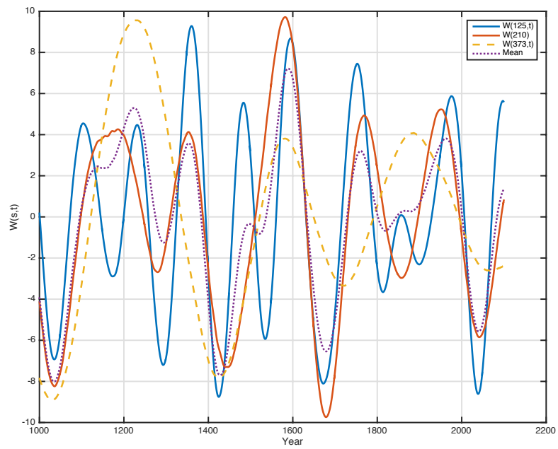
Figure 9: Identified long stationary wavelet periods Wls(125, t) , Wls(210, t) , Wls(373, t) and their mean value
