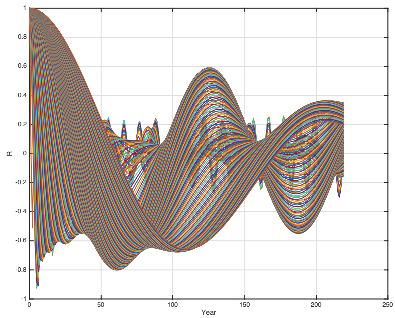
Figure 8: Autocorrelations Rls(s, m) of the TSI-LS wavelet spectrum Wls(s, t) for s = 0 \dots 600 , and m = 0 \dots 225 .
