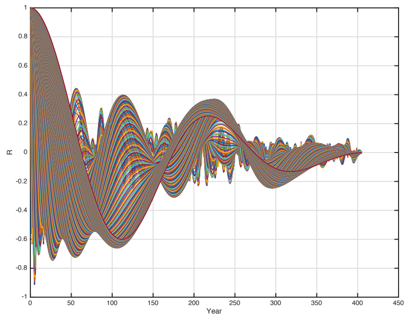
Figure 12: Autocorrelations Rsn(s, m) of the SN wavelet spectrum Wsn(s, t) for s = 0 \dots 240 , and m = 0 \dots 400 .
