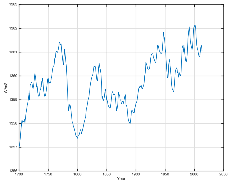
Figure 3: TSI-HS total solar irradiance from A.D. 1700 to 2013 (Scafetta & Willson, 2014).
