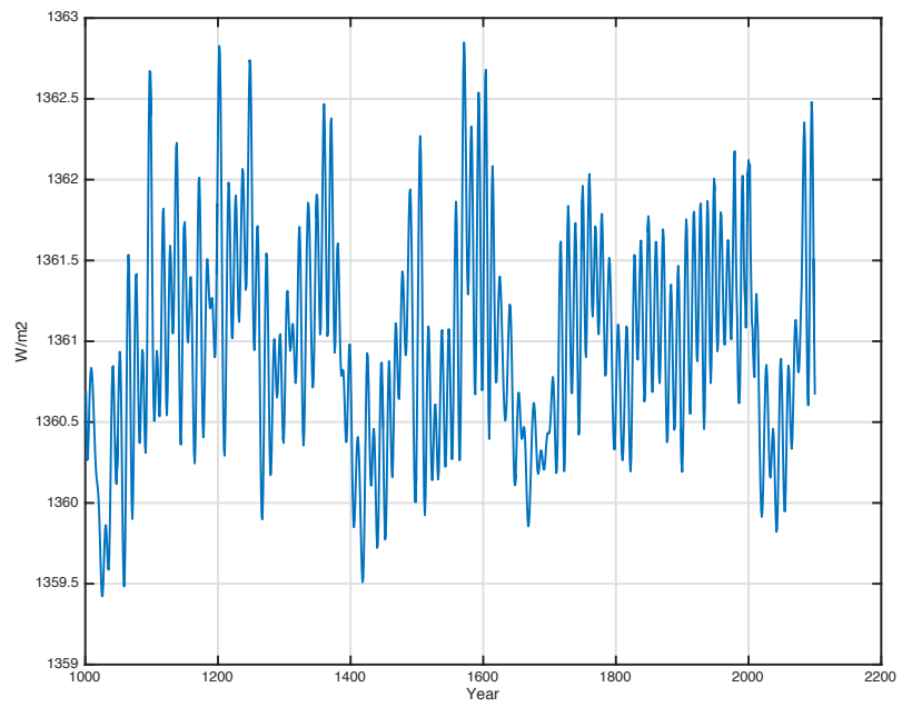
Figure 7: TSI-LS data series from 1000 to 2100 Velasco Herrera et al. (2015).
