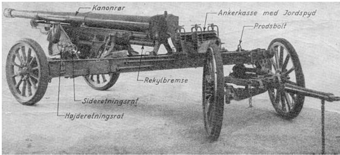
15 cm L/17 S.H. M.1917 (15 cm 17 kaliber lang stålhaubits Model 1917)
