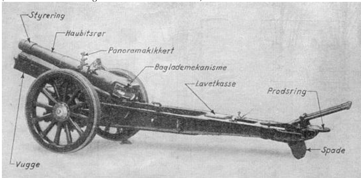
15 cm L/17 S.H. M.1917 (15 cm 17 kaliber lang stålhaubits Model 1917)
