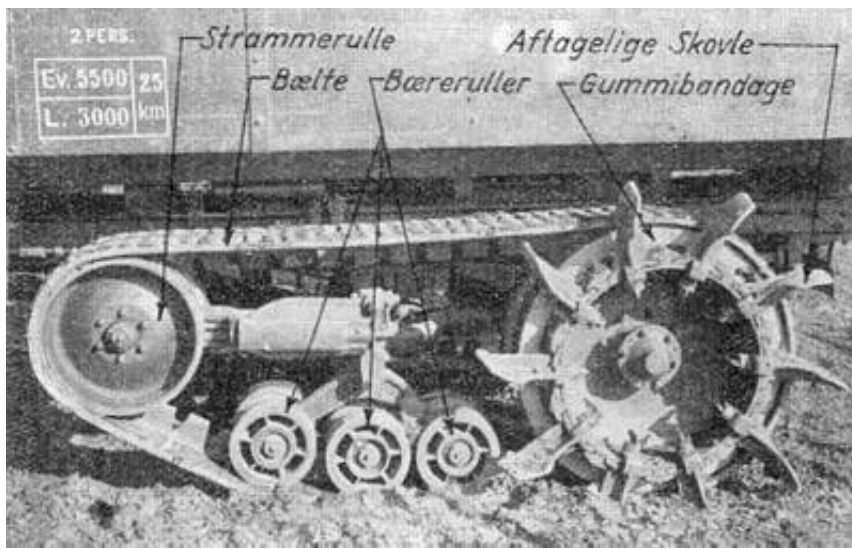
Artilleritraktor, Triangel
