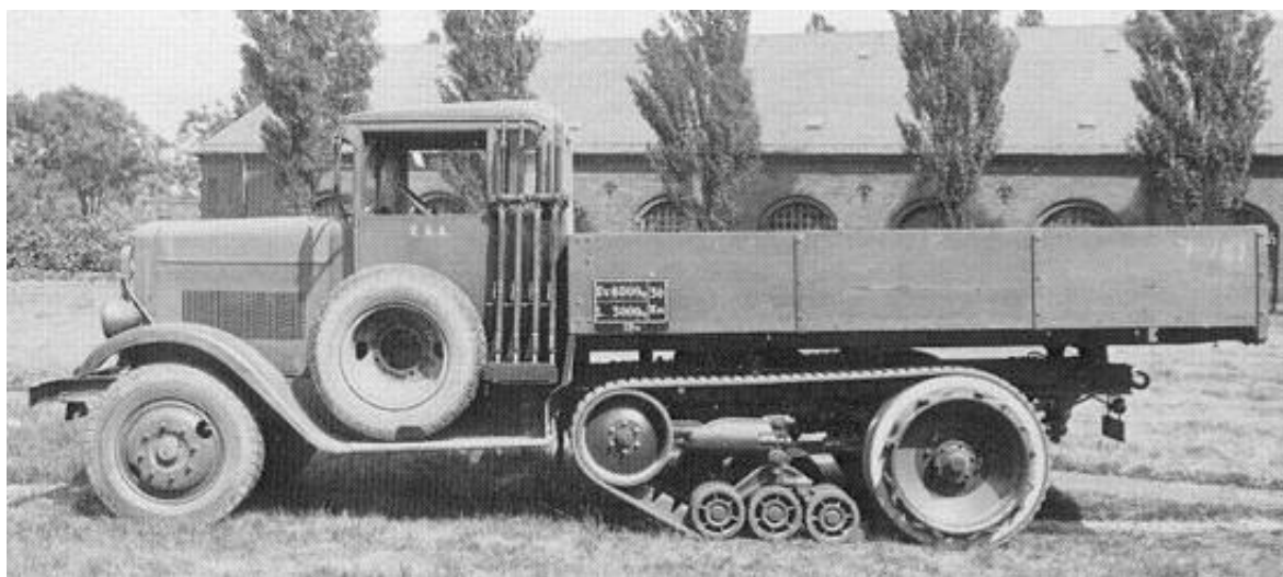
Artilleritraktor, Triangel
