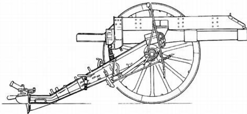
Carriage - BLC 15-pdr Field Gun Mk. 1. Fra Kilde 7.
