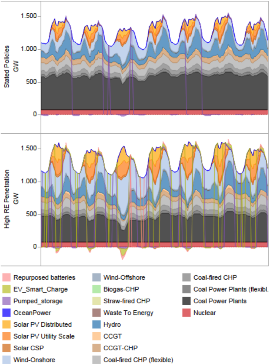
Figure 31: Hourly dispatch of China's national power supply and storage in a sample week (12) in 2030 in the two scenarios.
