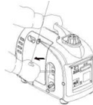
STARTSPAKE
