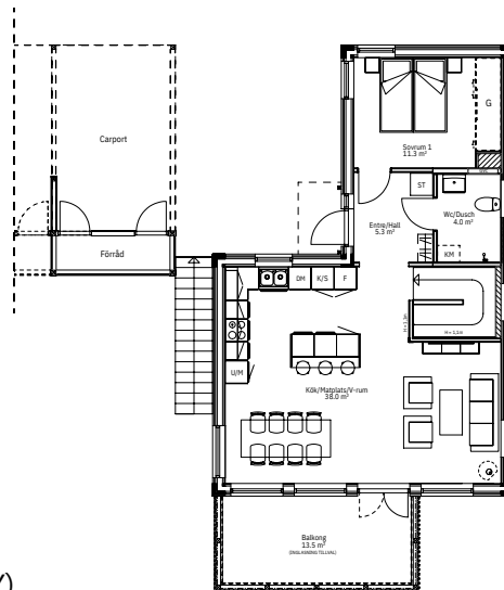
Plan 1
