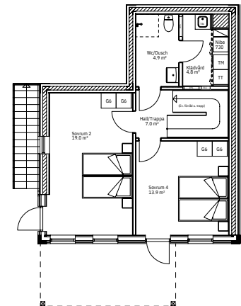
Plan 0
