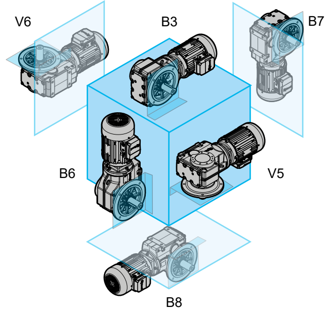
FE - flange mounted design
