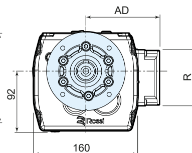
UTC 2404
