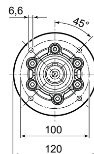
UTC 2405
