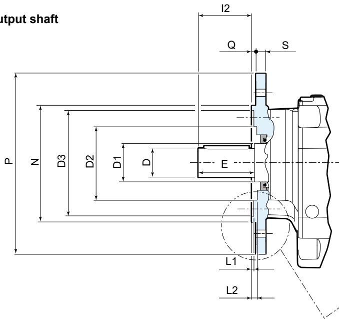
Details of gearmotor fastening flanges
