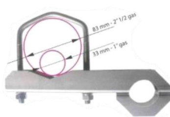
Fixing brackets
