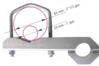
Fixing brackets
