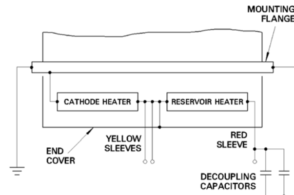
Fig. 1 CX1836 base connections
