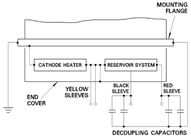
Fig. 2 CX1836X base connections
